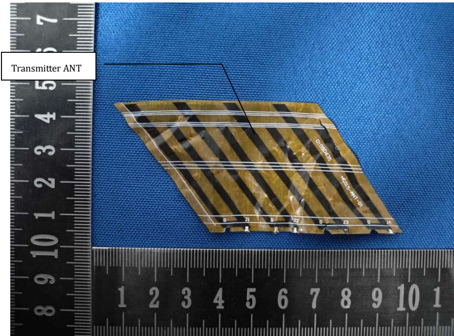
EUT Internal View 8
