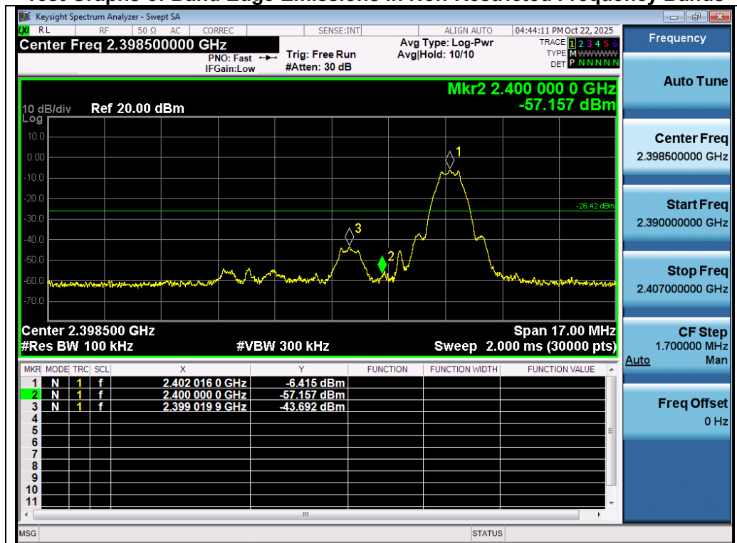
Test_Graph_SRD_ANT1_2402_2.4G_Lower Band Edge Emissions
