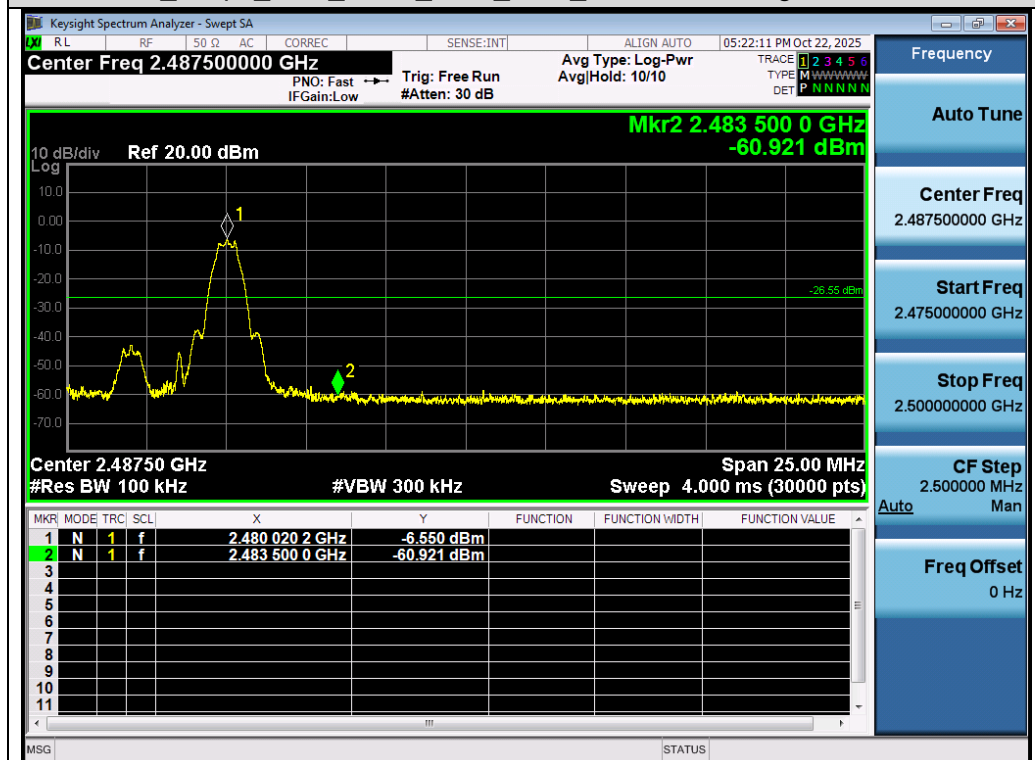
Test_Graph_SRD_ANT1_2480_2.4G_Higher Band Edge Emissions
