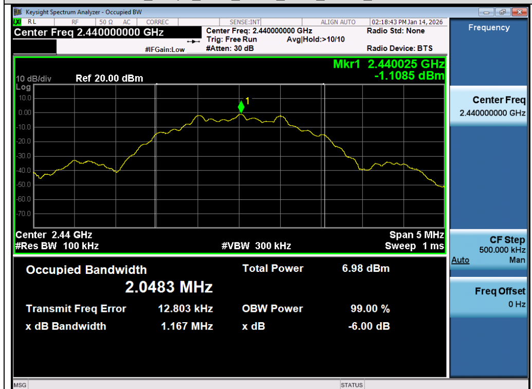
Test_Graph_2.4G_ANT1_2440_GFSK_DTSBW
