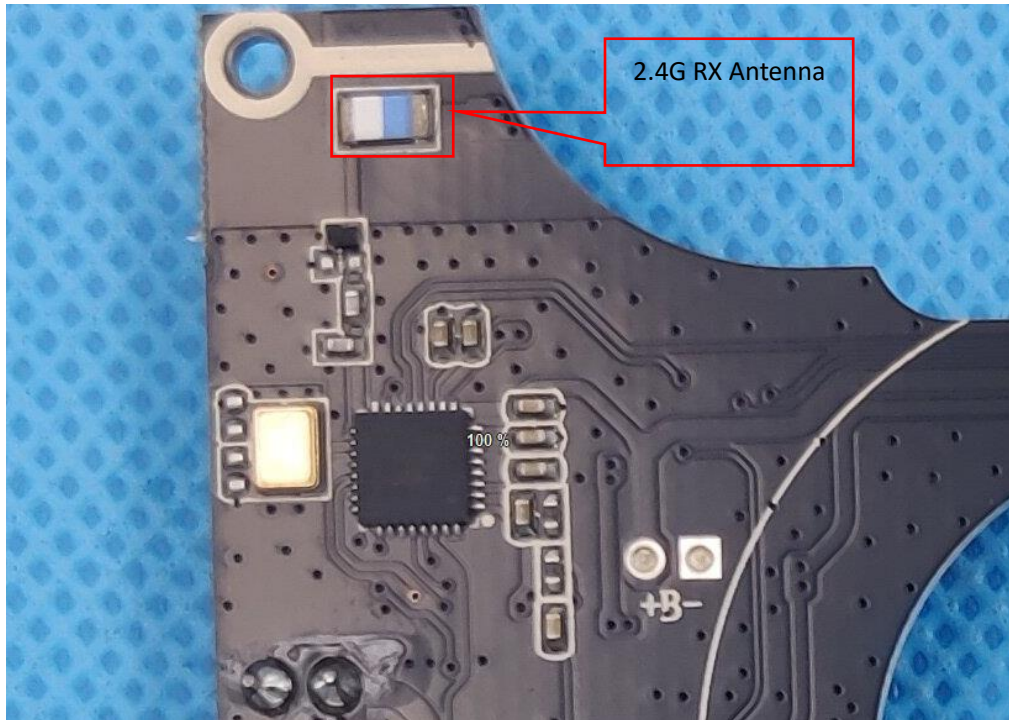
Internal view-3 of EUT
