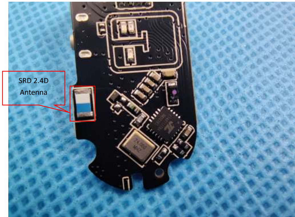
Internal view-3 of EUT
