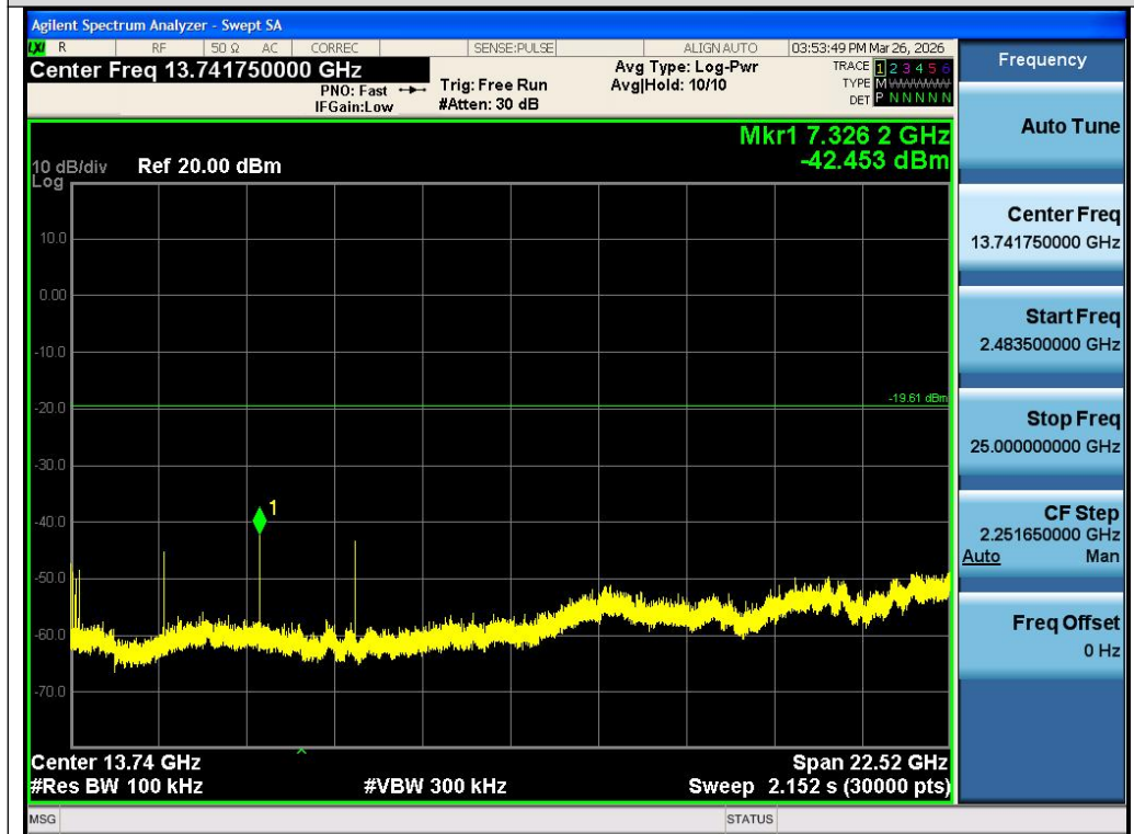
Test_Graph_2.4G_SRD_ANT1_2440_1Mbps_Higher Band Emissions
