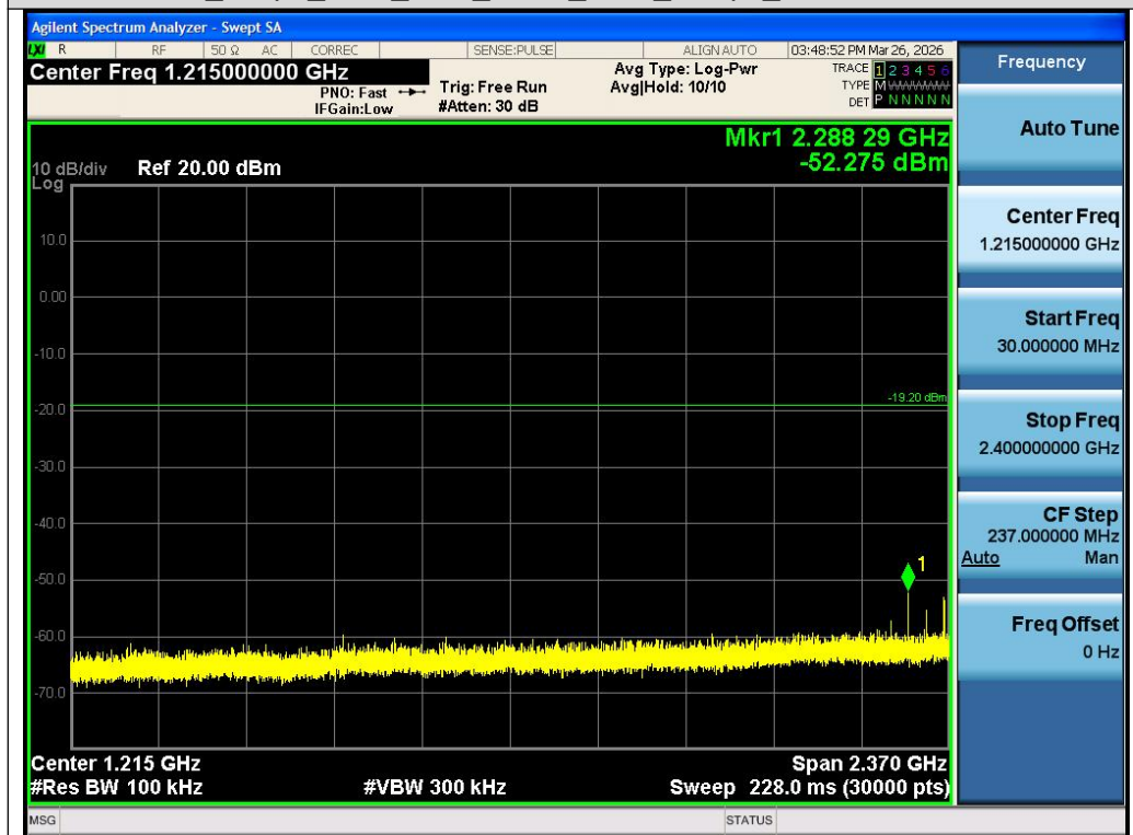
Test_Graph_2.4G_SRD_ANT1_2480_1Mbps_Lower Band Emissions
