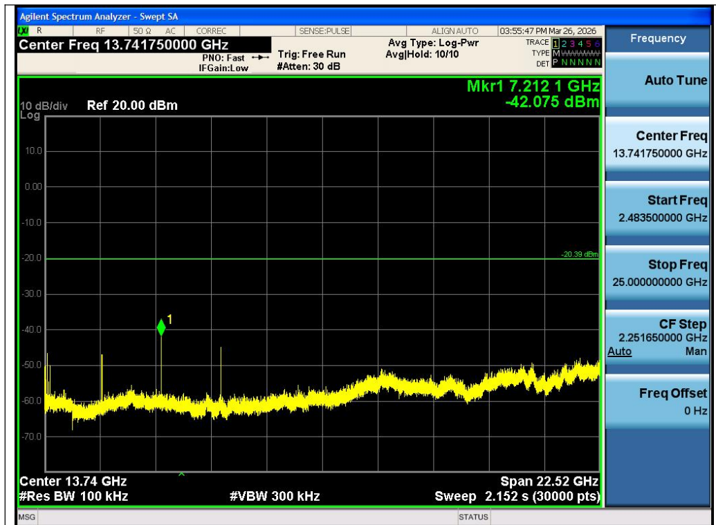
Test_Graph_2.4G_SRD_ANT1_2402_1Mbps_Higher Band Emissions
