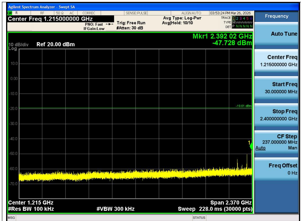
Test_Graph_2.4G_SRD_ANT1_2440_1Mbps_Lower Band Emissions
