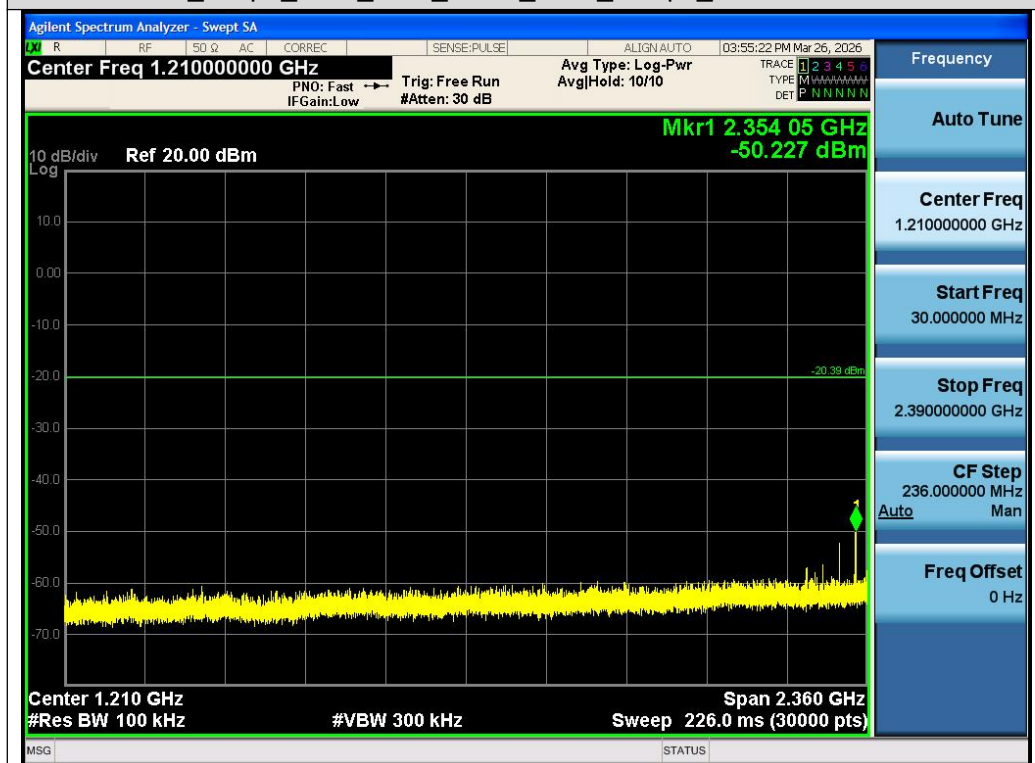
Test_Graph_2.4G_SRD_ANT1_2402_1Mbps_Lower Band Emissions
