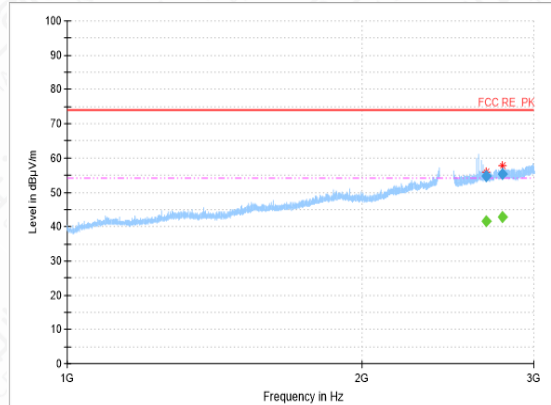
RSE-11N(20M)-CH1-1GHz-3GHz
