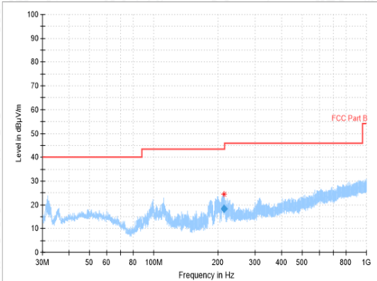
RSE-11N(20M)-CH1-30MHz-1GHz
