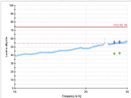
RSE-11N(20M)-CH11-1GHz-3GHz
