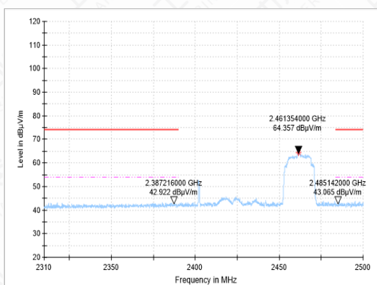
Bandedge-11N(20M)-CH11-AV
