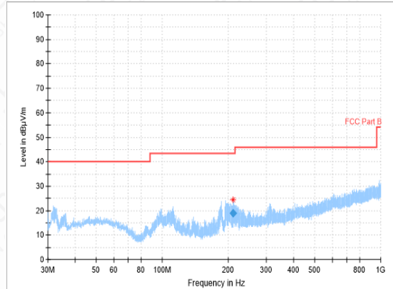
RSE-11N(20M)-CH11-30MHz-1GHz
