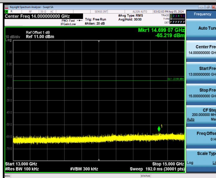
11G_Ant1_2437_15000~17000
