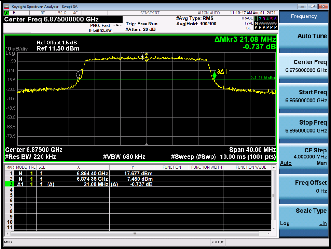
11AX20SISO-Ant1-6875
