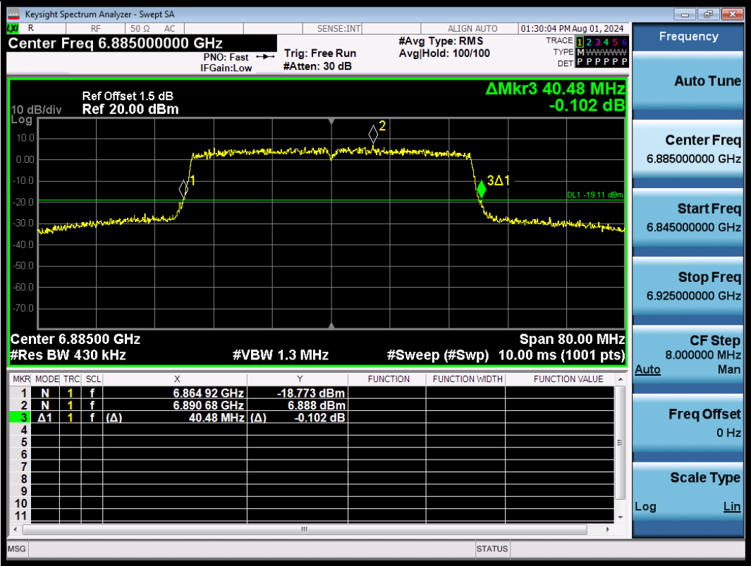
11AX40SISO-Ant1-6885
