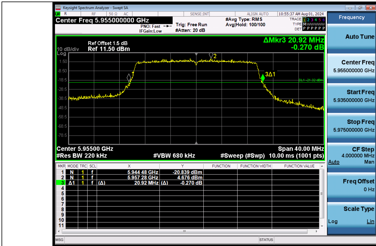
11AX20SISO-Ant1-5955
