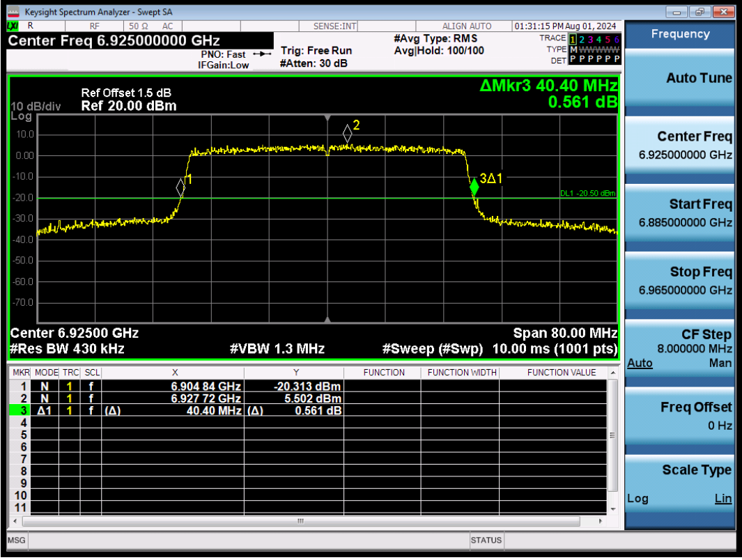
11AX40SISO-Ant1-6925
