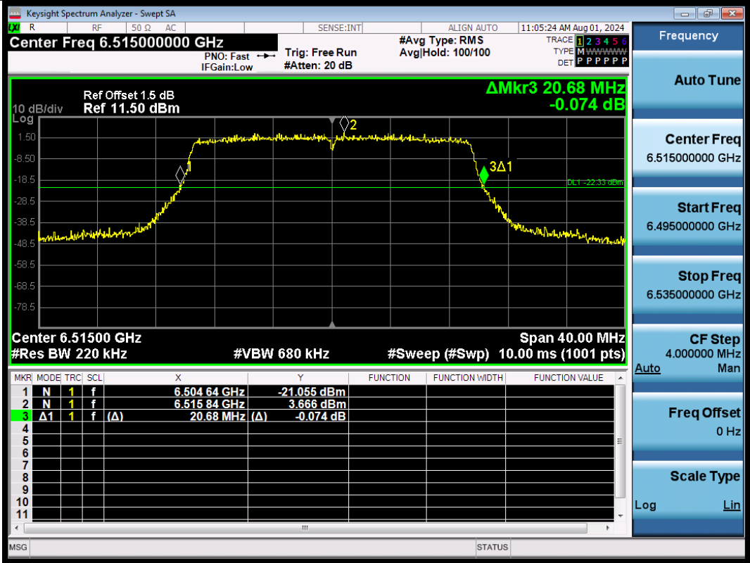
11AX20SISO-Ant1-6515
