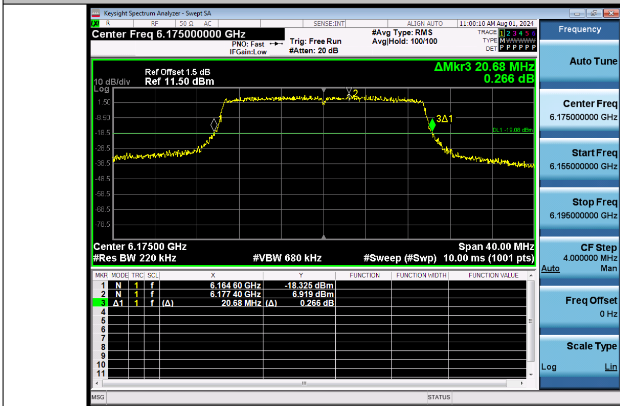
11AX20SISO-Ant1-6175
