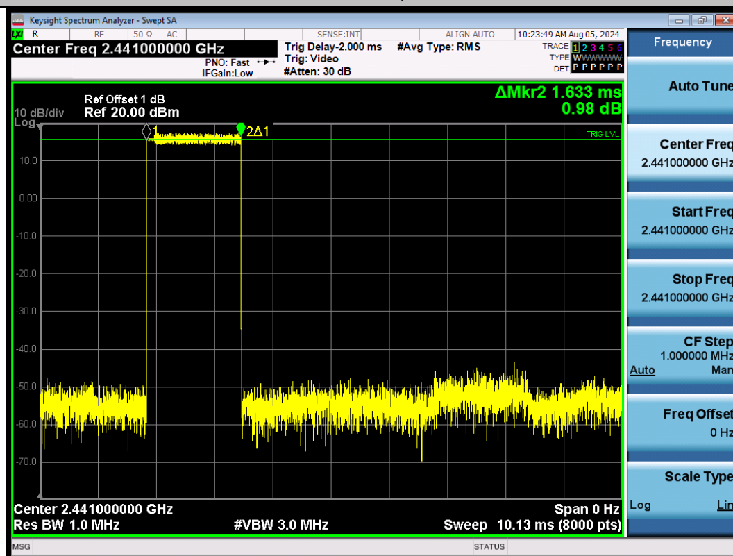
2DH3-Ant1-Hop-PASS
