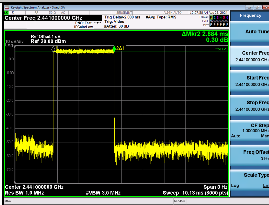
3DH5-Ant1-Hop-PASS
