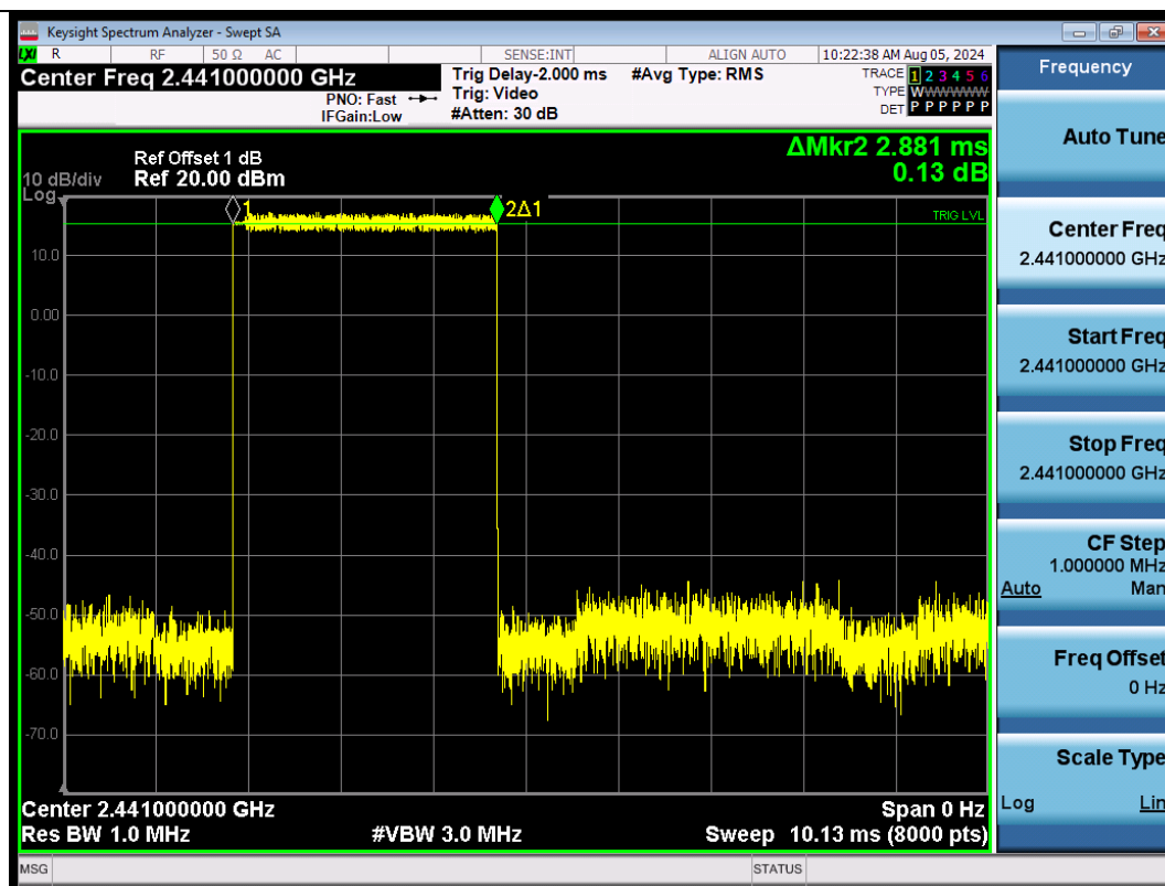
2DH5-Ant1-Hop-PASS
