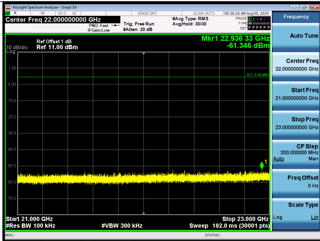
DH5-Ant1-2402-21000~23000-PASS
