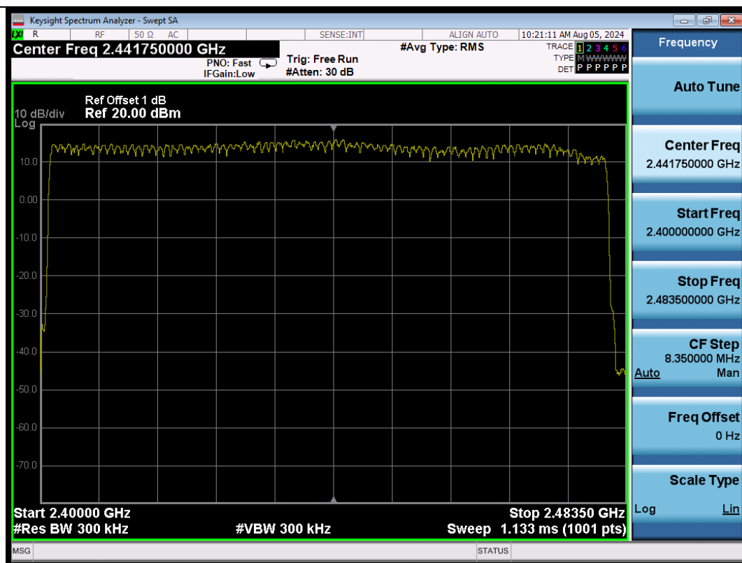
2DH5-Ant1-Hop-PASS
