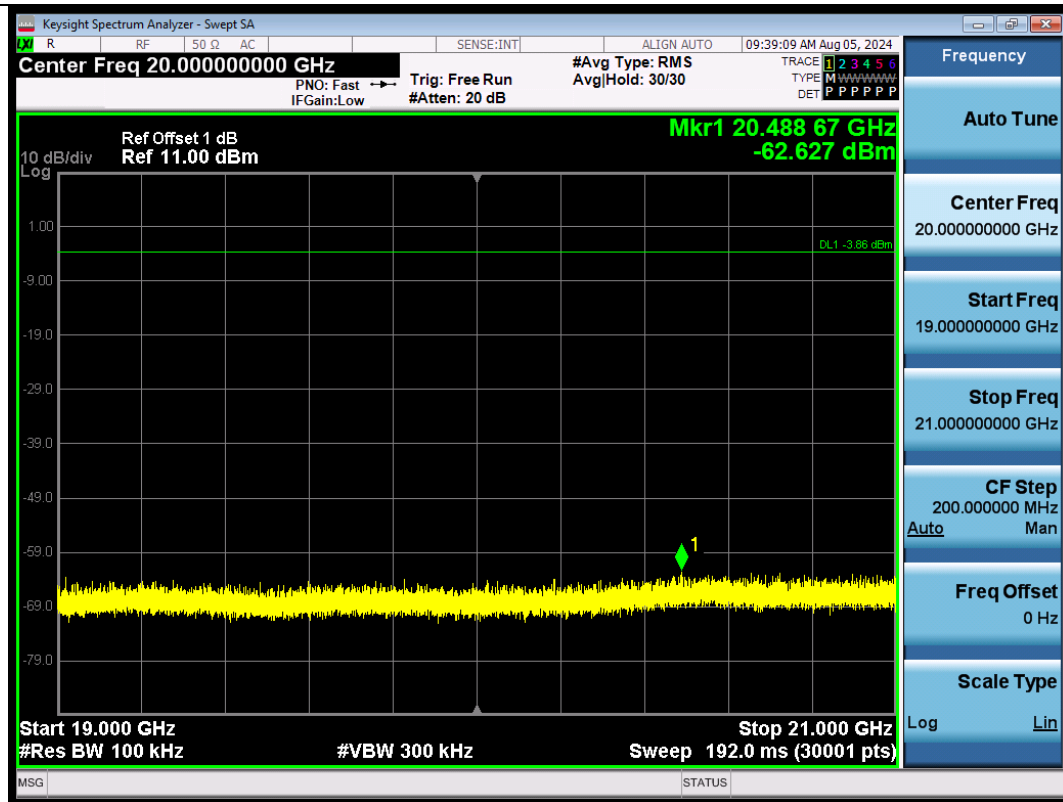
DH5-Ant1-2441-19000~21000-PASS
