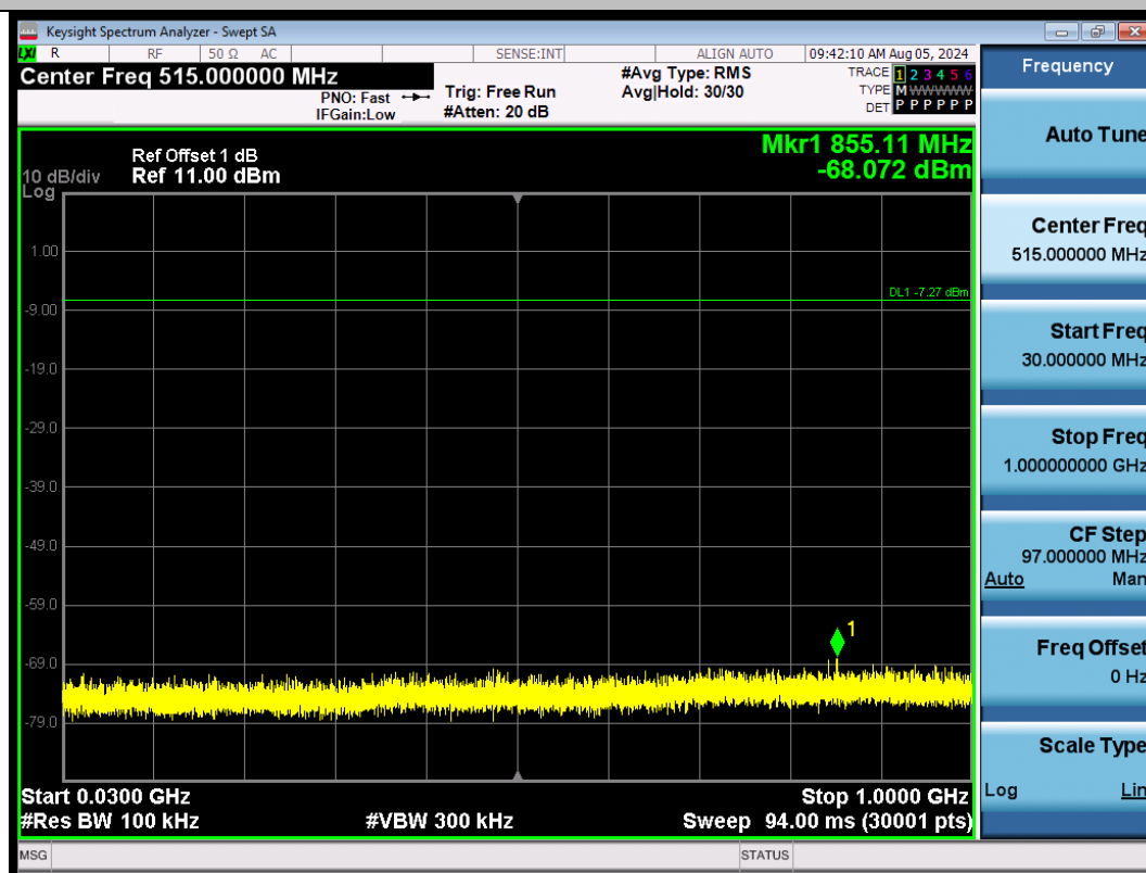
DH5-Ant1-2480-30~1000-PASS
