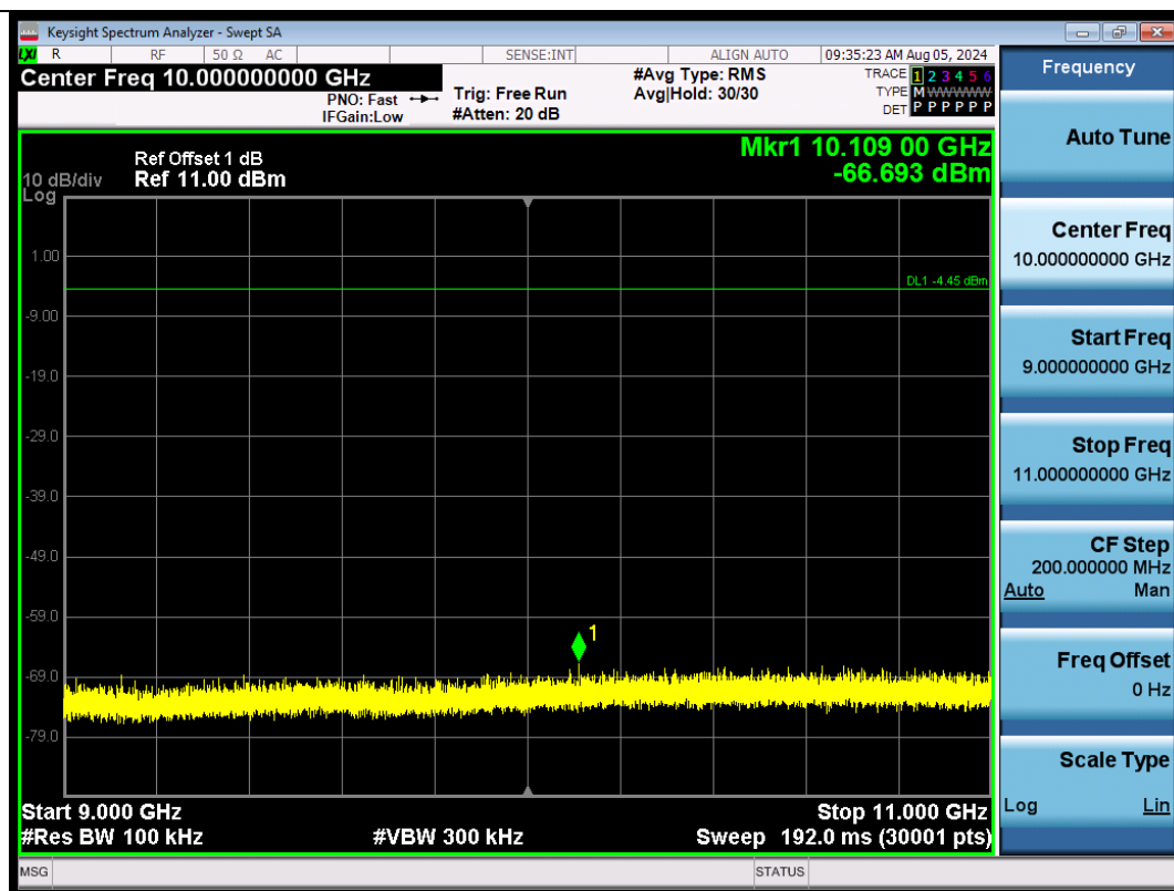
DH5-Ant1-2402-9000~11000-PASS
