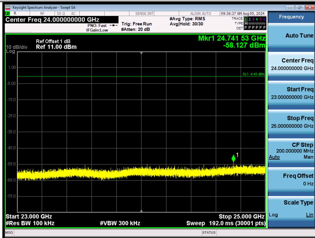
DH5-Ant1-2402-23000~25000-PASS
