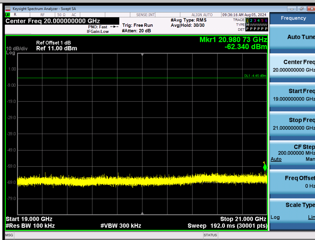
DH5-Ant1-2402-19000~21000-PASS
