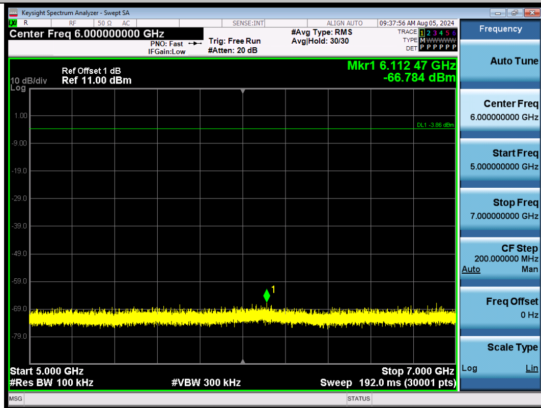
DH5-Ant1-2441-5000~7000-PASS
