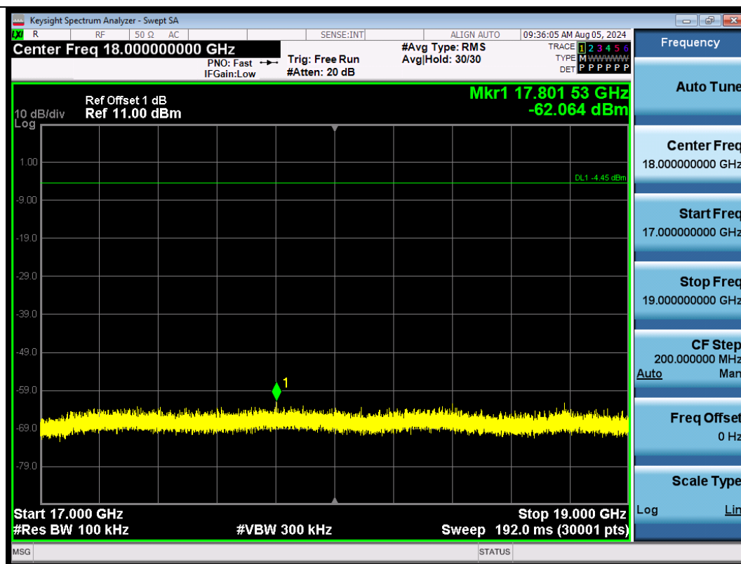
DH5-Ant1-2402-17000~19000-PASS
