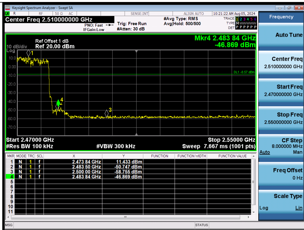
2DH5-Ant1-Hop_2480-PASS
