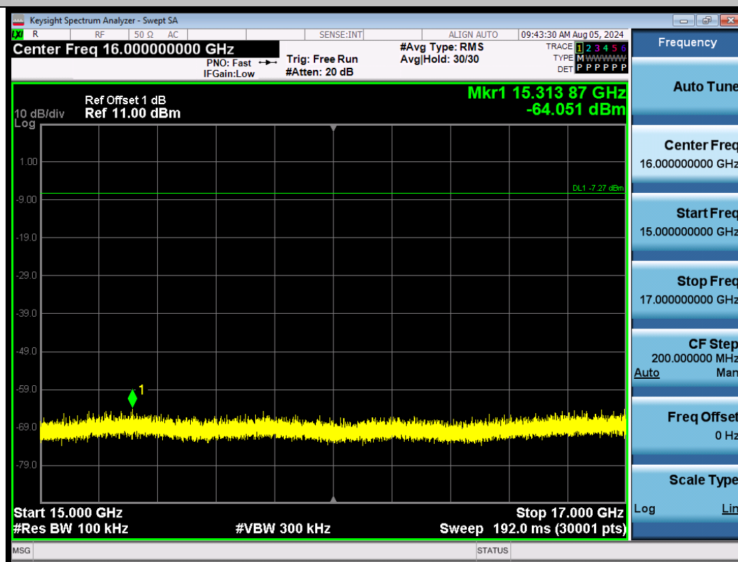
DH5-Ant1-2480-15000~17000-PASS
