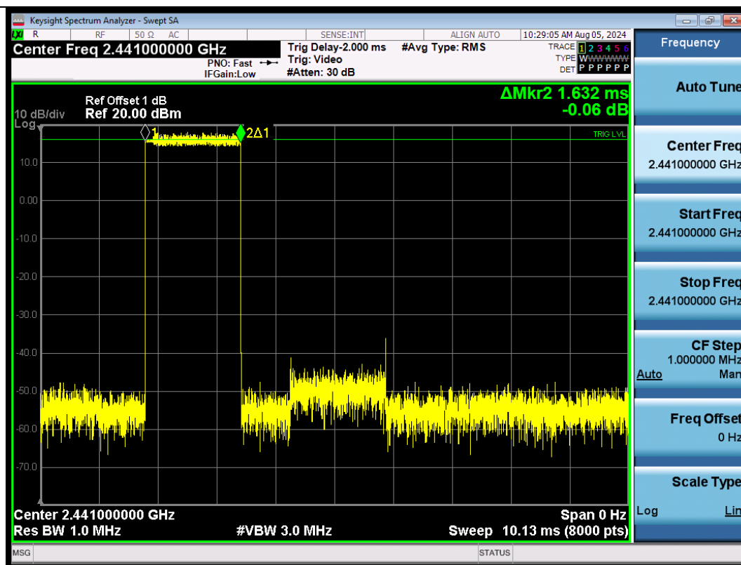
3DH3-Ant1-Hop-PASS
