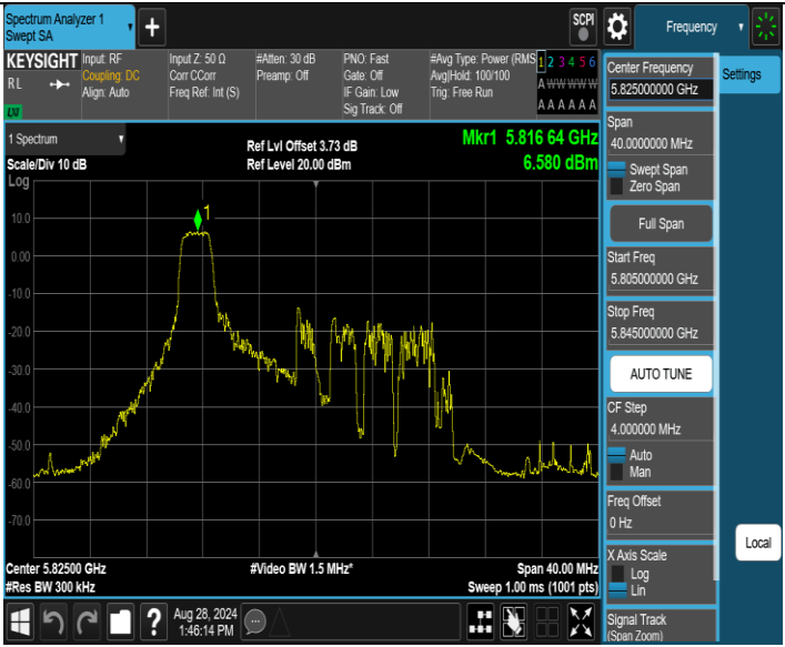
11AX20SISO_Ant1_5825_52Tone_RU37
