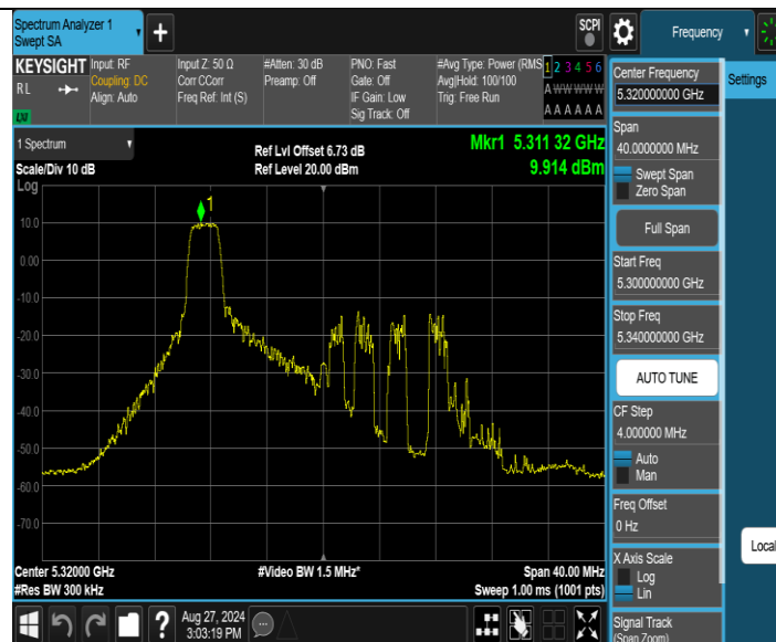
11AX20SISO_Ant1_5320_52Tone_RU37
