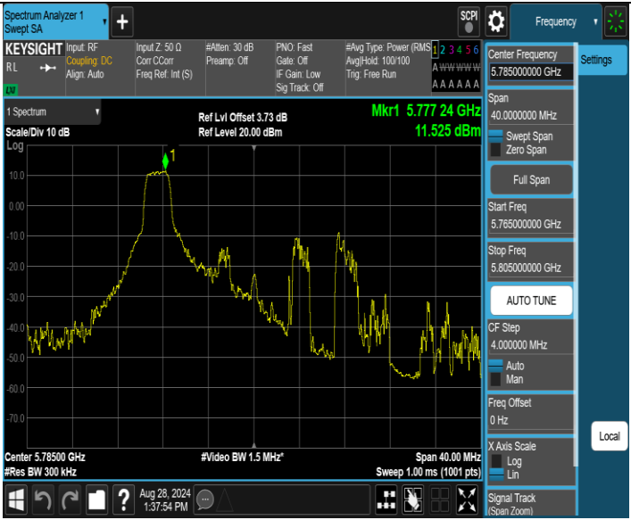
11AX20SISO_Ant1_5785_52Tone_RU37
