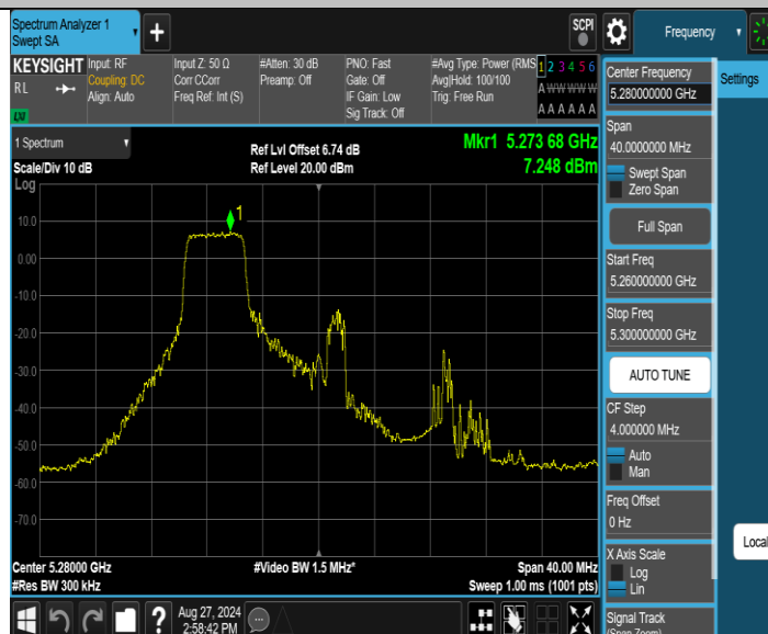
11AX20SISO_Ant1_5280_106Tone_RU53
