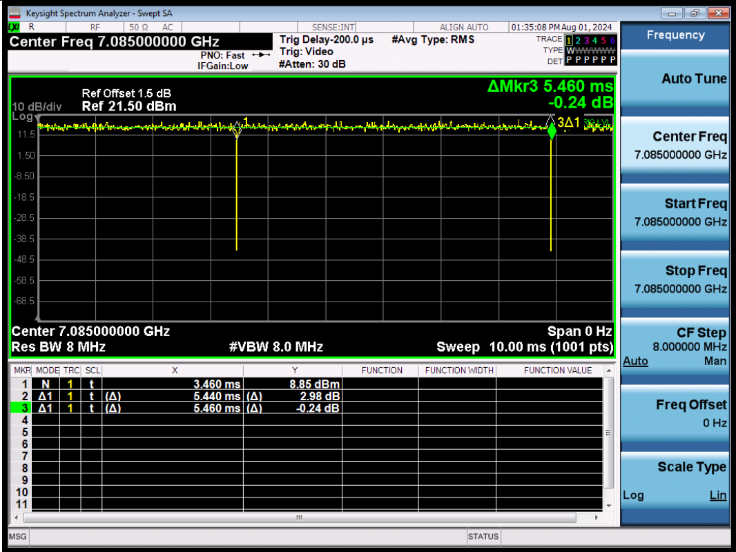
NTNV-11AX40SISO-Ant1-7085
