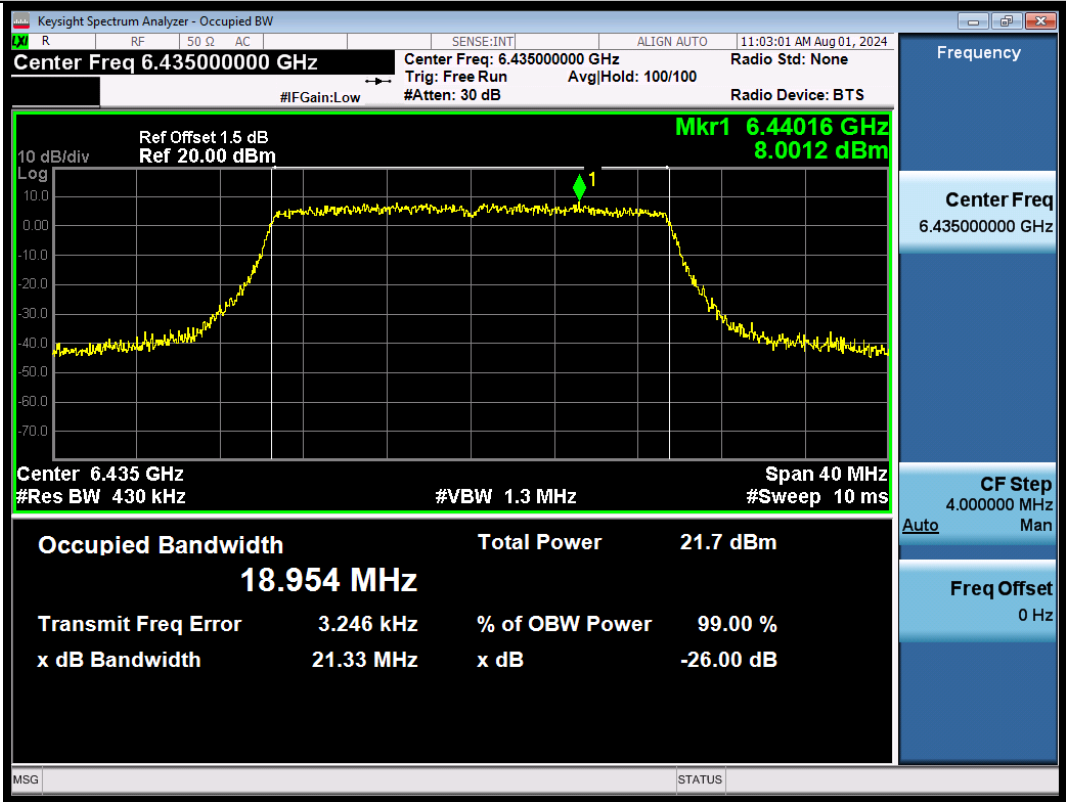
11AX20SISO-Ant1-6435-PASS
