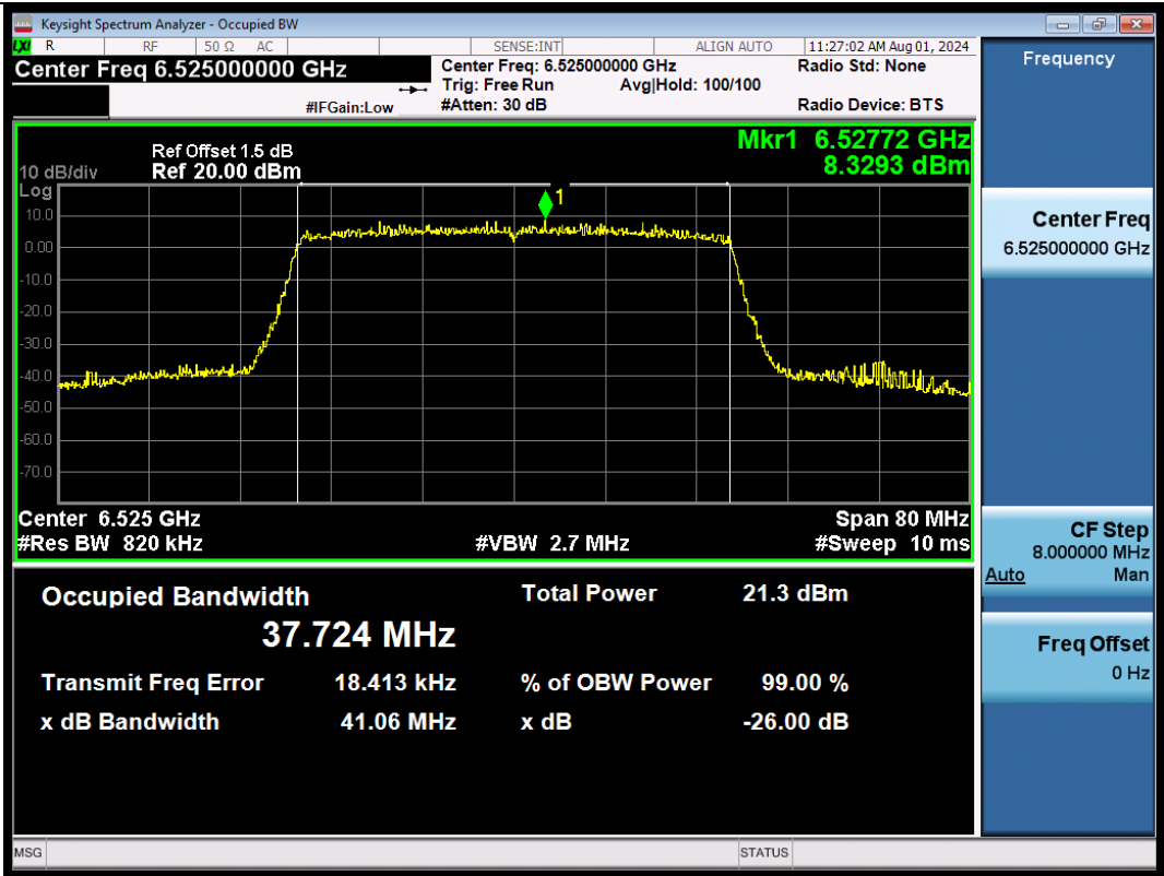
11AX40SISO-Ant1-6525-PASS
