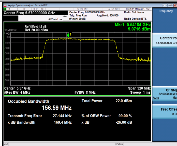
11AX160SISO_Ant1_5570
