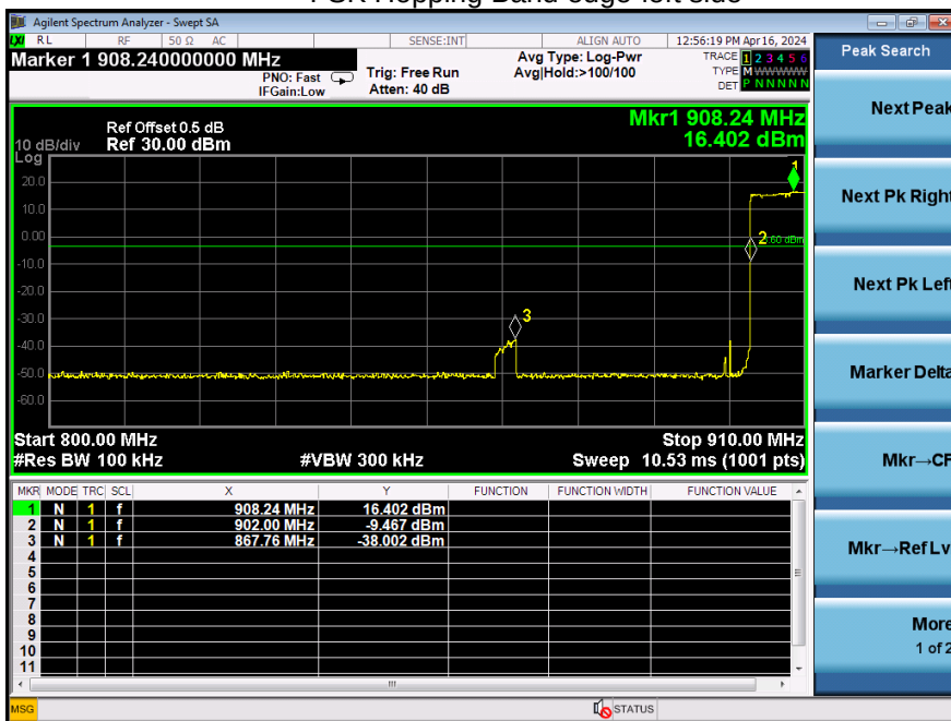
FSK Hopping Band edge-left side
