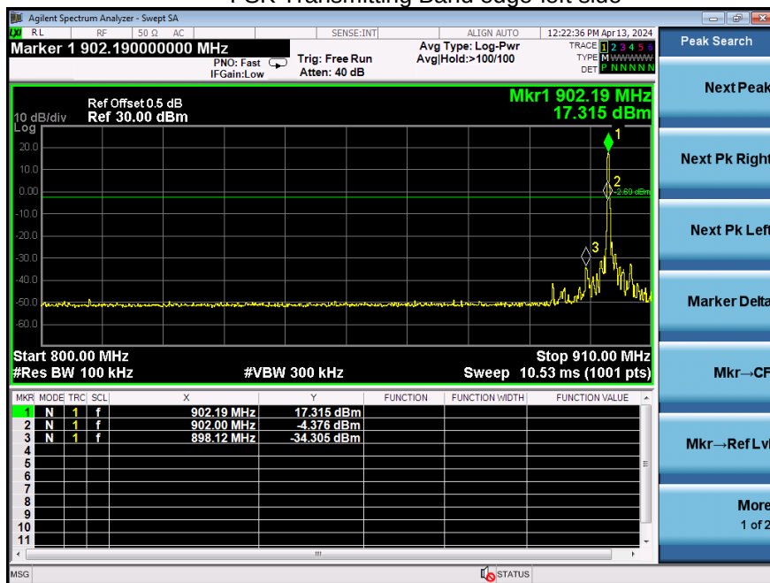
FSK Transmitting Band edge-left side
