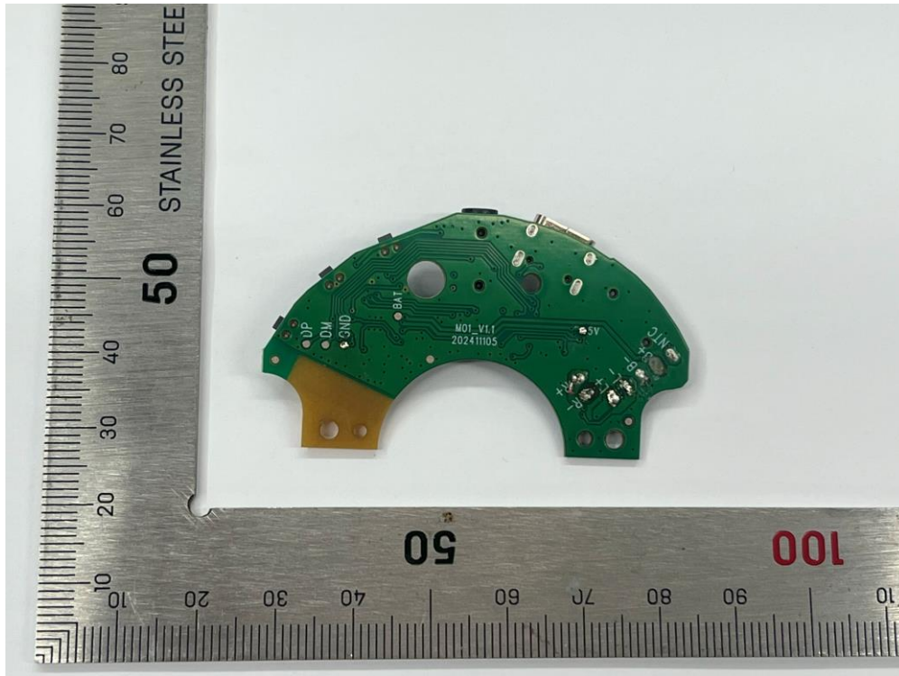
Fig. 3 PCB view
