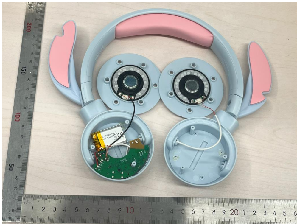
Fig. 1 Internal view
