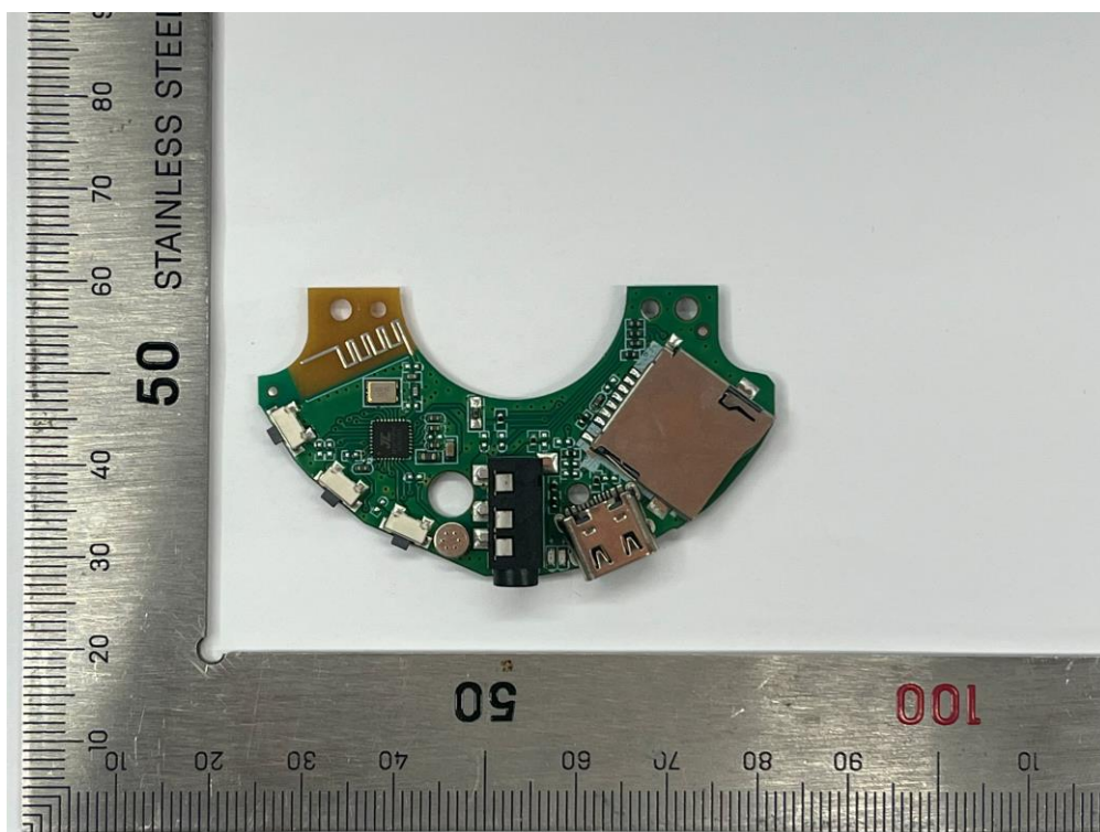
Fig. 2 Internal view
