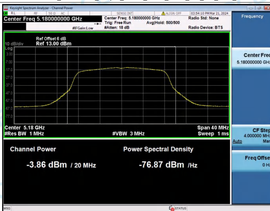
Maximum_Conducted_Output_Power_NVNT_ANT1_802_11a_5180_20M
