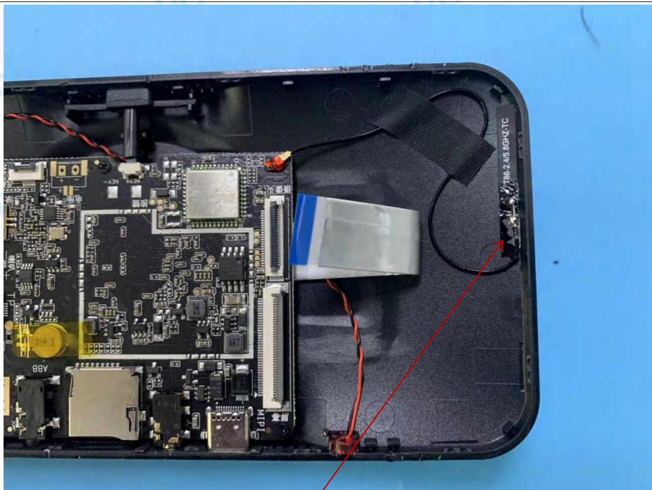
WIFI-ANT
