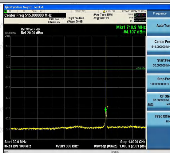
Band12_1.4MHz_16QAM_23173_1RB#0_30~1000_30~1 000
