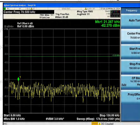
Band12_1.4MHz_16QAM_23173_1RB#0_0.009~0.15_0.0 09~0.15
