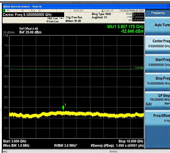
Band12_1.4MHz_QPSK_23173_1RB#0_3000~10000_3 000~10000
