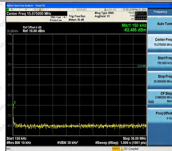
Band12_1.4MHz_QPSK_23173_1RB#0_0.15~30_0.15~3 0
