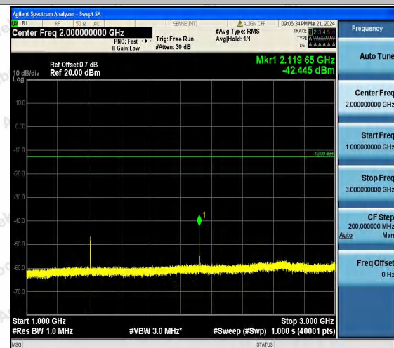
Band12_10MHz_QPSK_23130_1RB#0_1000~3000_1000 ~3000
