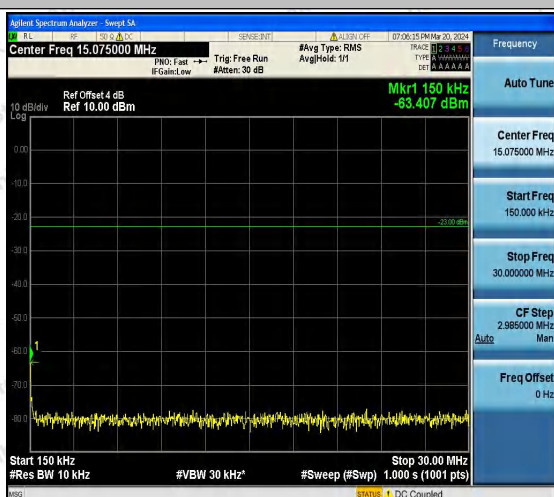
Band12_1.4MHz_16QAM_23173_1RB#0_0.15~30_0.15 ~30
