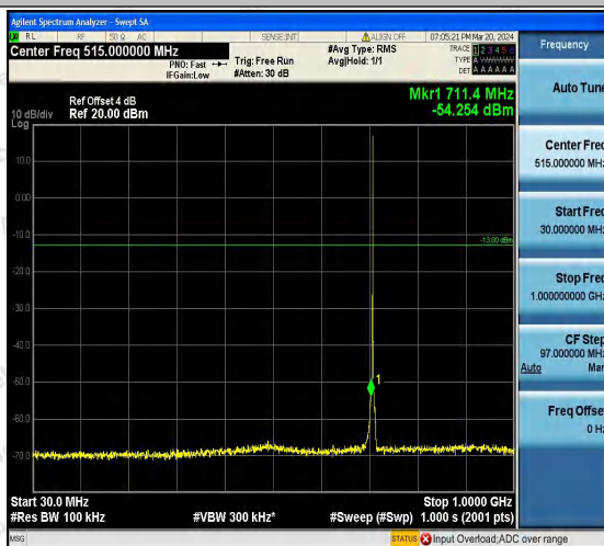
Band12_1.4MHz_QPSK_23173_1RB#0_30~1000_30~1 000
