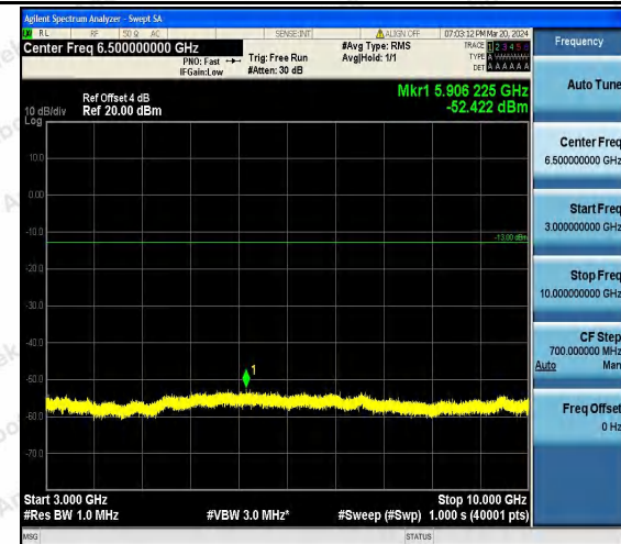
Band12_1.4MHz_16QAM_23095_1RB#0_3000~10000_3 000~10000
