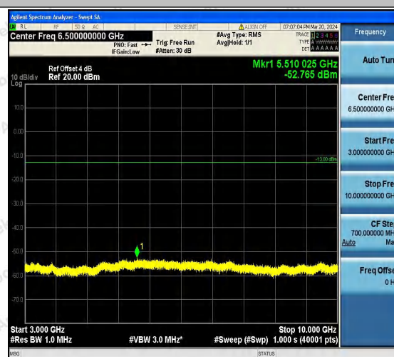
Band12_1.4MHz_16QAM_23173_1RB#0_3000~10000_3 000~10000
