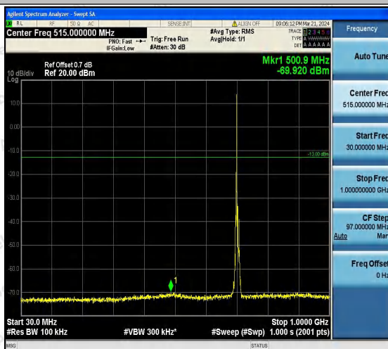
Band12_10MHz_QPSK_23130_1RB#0_30~1000_30~10 00
