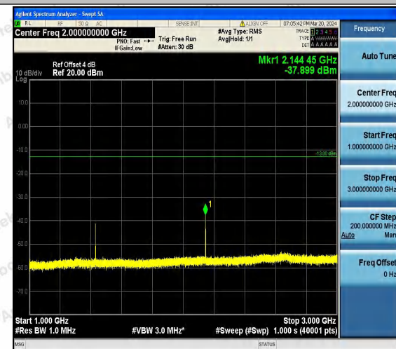
Band12_1.4MHz_QPSK_23173_1RB#0_1000~3000_100 0~3000
