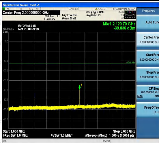
Band12_1.4MHz_16QAM_23095_1RB#0_1000~3000_1 000~3000
