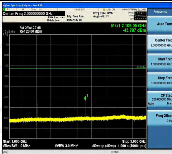
Band12_10MHz_16QAM_23095_1RB#0_1000~3000_10 00~3000
