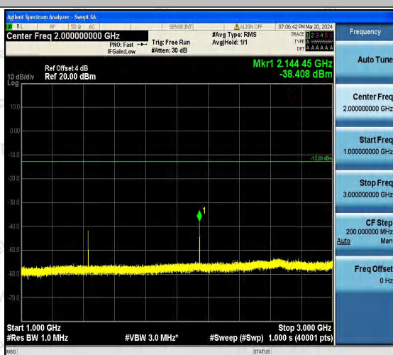
Band12_1.4MHz_16QAM_23173_1RB#0_1000~3000_1 000~3000
