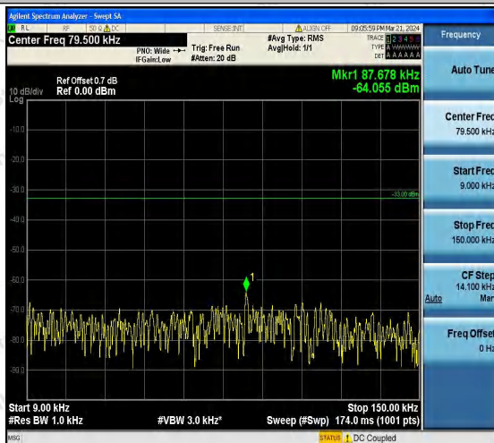
Band12_10MHz_QPSK_23130_1RB#0_0.009~0.15_0.0 09~0.15
