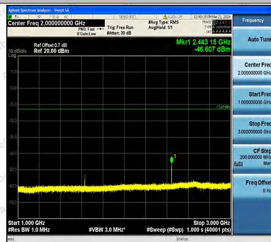
Band26_5MHz_QPSK_26715_1RB#0_1000~3000_1000 ~3000
