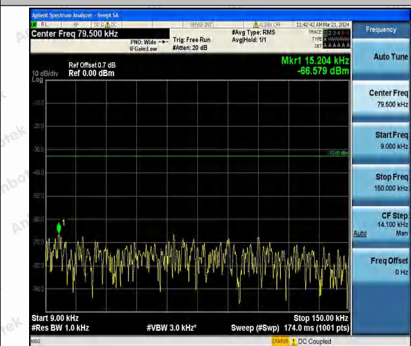
Band26_1.4MHz_16QAM_26697_1RB#0_0.009~0.15_0.009~0.15
