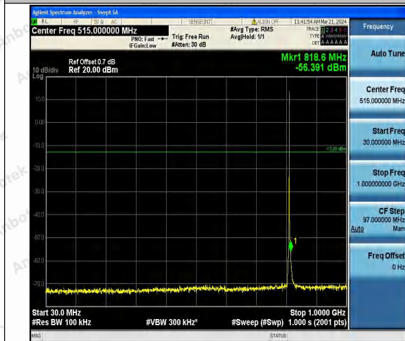
Band26_1.4MHz_QPSK_26697_1RB#0_30~1000_30~1000
