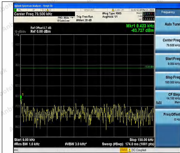
Band26_1.4MHz_QPSK_26697_1RB#0_0.009~0.15_0.009~0.15
