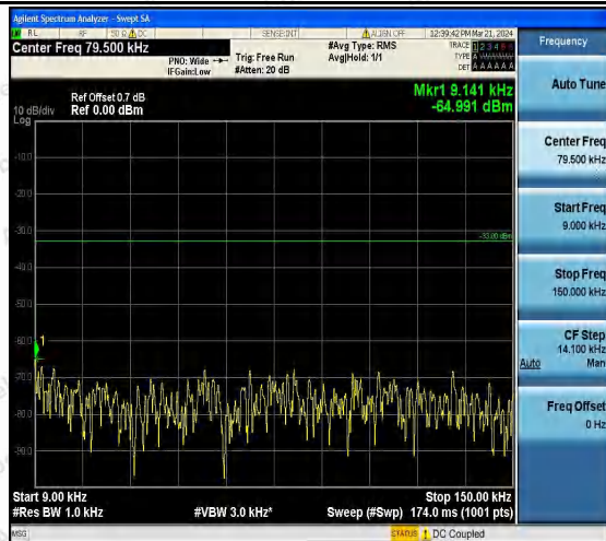
Band26_5MHz_QPSK_26715_1RB#0_0.009~0.15_0.0 09~0.15
