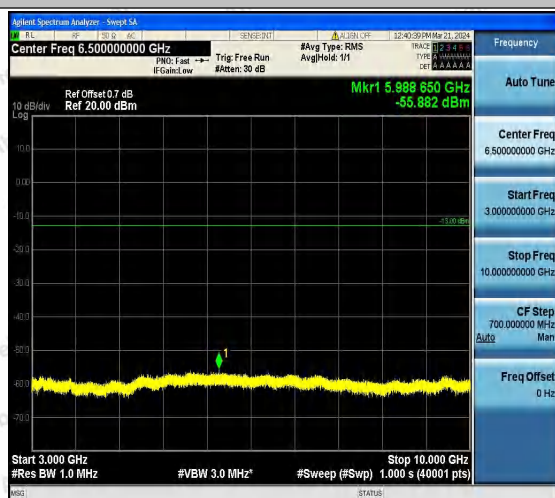
Band26_5MHz_QPSK_26715_1RB#0_3000~10000_30 00~10000
