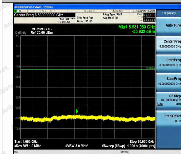
Band26_1.4MHz_QPSK_26697_1RB#0_3000~10000_3000~10000
