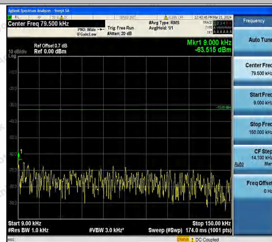
Band26_5MHz_16QAM_26715_1RB#0_0.009~0.15_0.0 09~0.15
