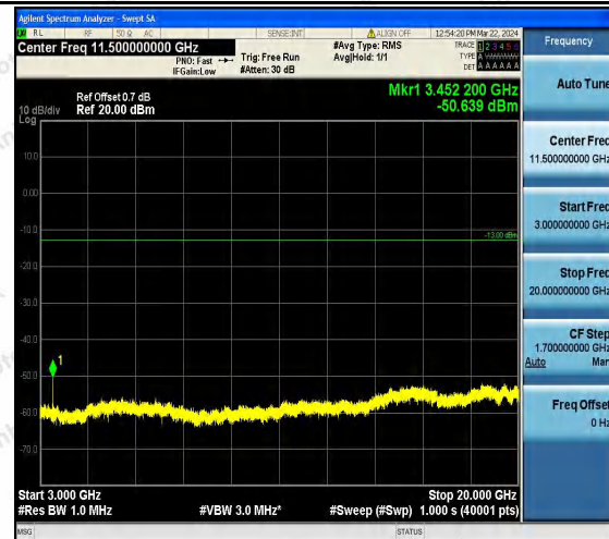
Band4_15MHz_16QAM_20175_1RB#0_3000~20000_3 000~20000
