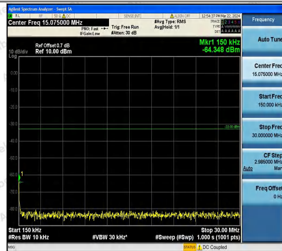
Band4_15MHz_QPSK_20325_1RB#0_0.15~30_0.15~30
