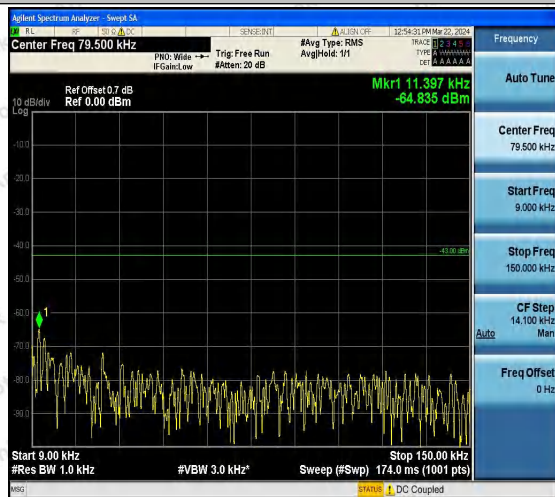
Band4_15MHz_QPSK_20325_1RB#0_0.009~0.15_0.0 09~0.15
