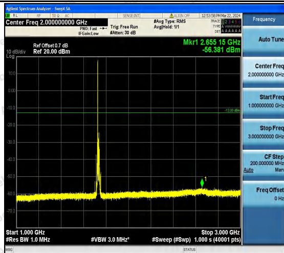
Band4_15MHz_16QAM_20175_1RB#0_1000~3000_10 00~3000
