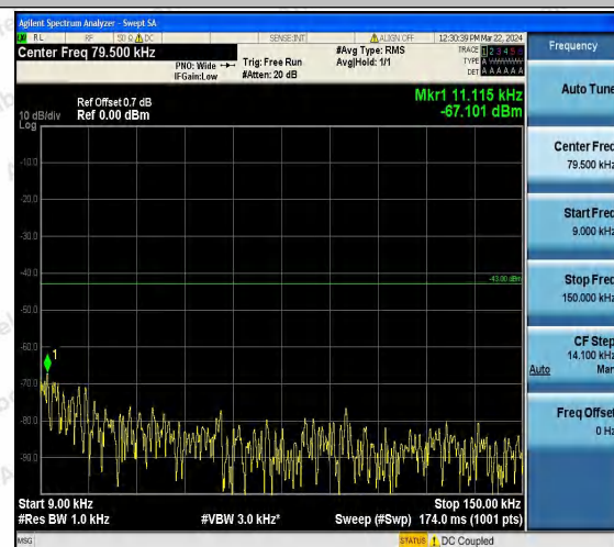
Band4_10MHz_16QAM_20175_1RB#0_0.009~0.15_0.0
