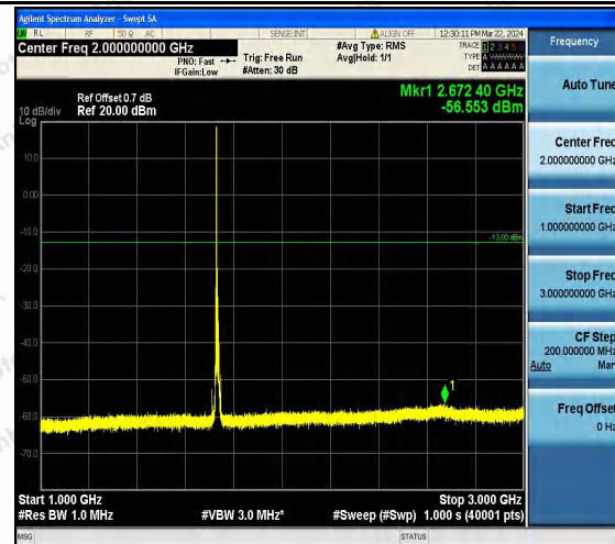
Band4_10MHz_QPSK_20175_1RB#0_1000~3000_1000
