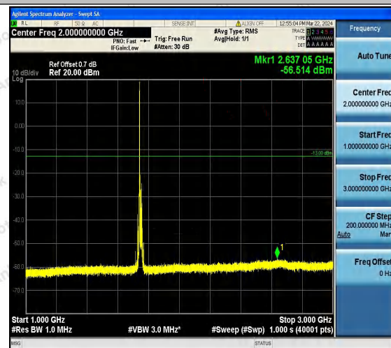
Band4_15MHz_QPSK_20325_1RB#0_1000~3000_1000 ~3000
