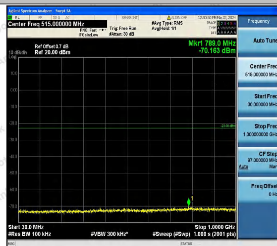
Band4_10MHz_16QAM_20175_1RB#0_30~1000_30~1
