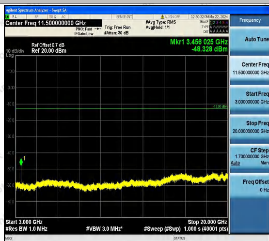
Band4_10MHz_QPSK_20175_1RB#0_3000~20000_30
