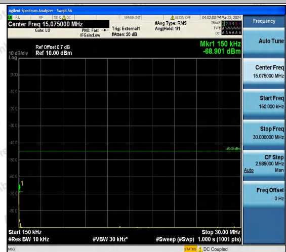
Band41_10MHz_16QAM_41190_1RB#0_0.15~30_0.15~30
