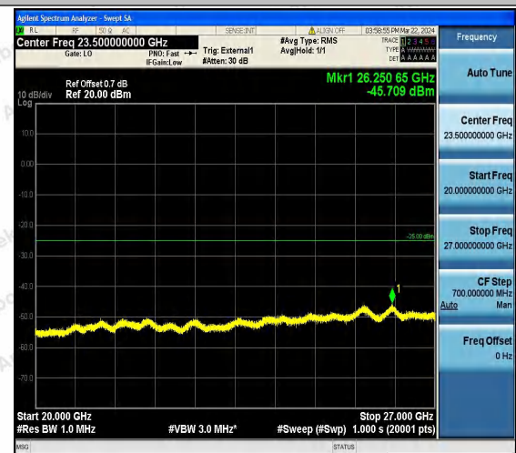
Band41_10MHz_QPSK_40590_1RB#0_20000~27000_20 000~27000
