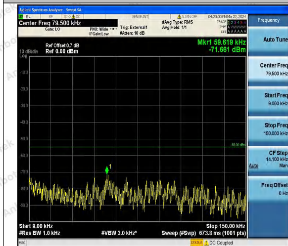
Band41_15MHz_16QAM_40115_1RB#0_0.009~0.15_ 0.009~0.15
