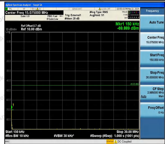
Band41_10MHz_QPSK_40090_1RB#0_0.15~30_0.15~30
