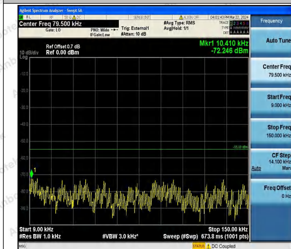
Band41_10MHz_16QAM_41190_1RB#0_0.009~0.15_0.009~0.15
