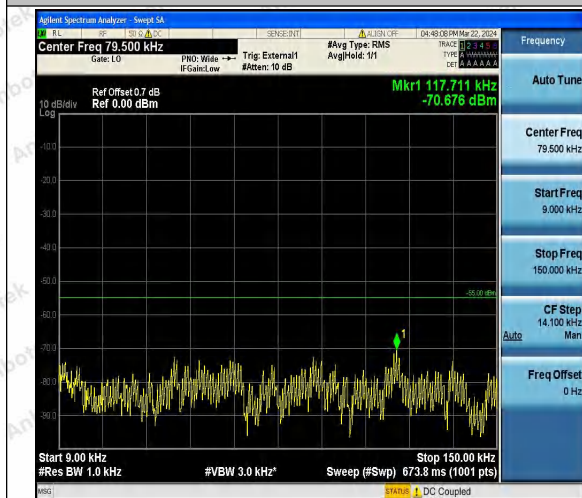
Band41_20MHz_QPSK_41140_1RB#0_0.009~0.15_0 .009~0.15
