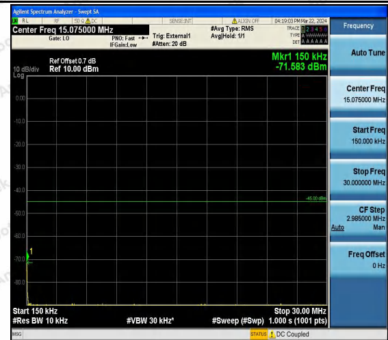
Band41_15MHz_QPSK_40115_1RB#0_0.15~30_0.15~30
