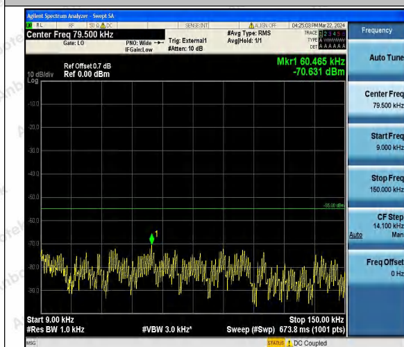
Band41_15MHz_16QAM_41165_1RB#0_0.009~0.15_0.009~0.15
