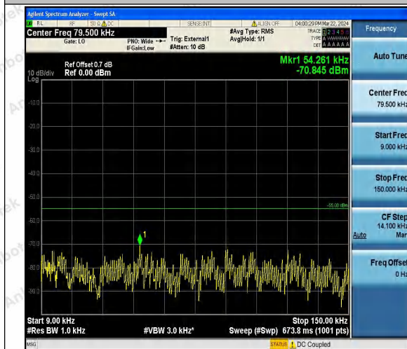
Band41_10MHz_QPSK_41190_1RB#0_0.009~0.15_0 .009~0.15
