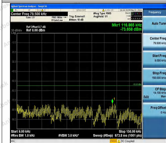
Band41_20MHz_16QAM_40140_1RB#0_0.009~0.15_0.009~0.15
