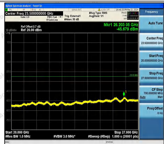
Band41_20MHz_QPSK_40590_1RB#0_20000~27000_20 000~27000
