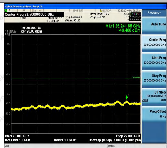
Band41_5MHz_QPSK_40590_1RB#0_20000~27000_200 00~27000
