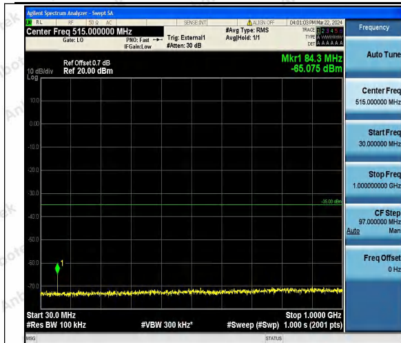
Band41_10MHz_QPSK_41190_1RB#0_30~1000_30~1000
