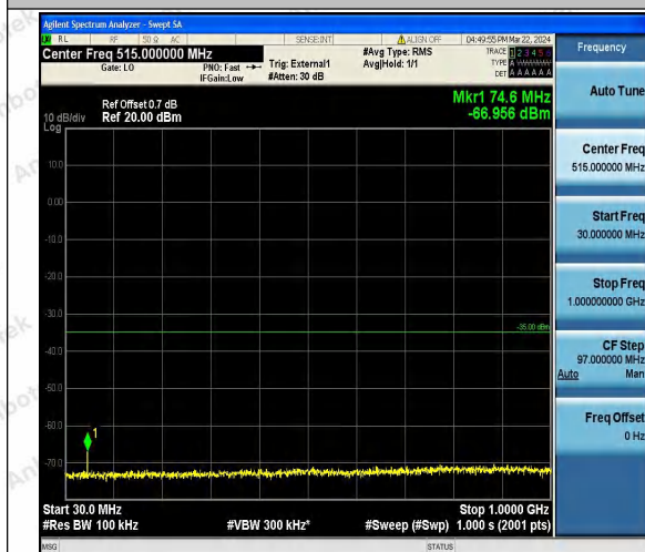
Band41_20MHz_16QAM_41140_1RB#0_30~1000_30~1000
