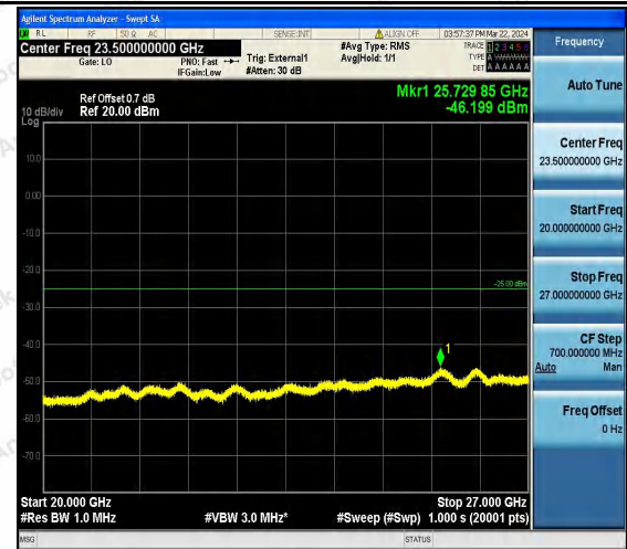
Band41_10MHz_16QAM_40090_1RB#0_20000~27000_2 0000~27000
