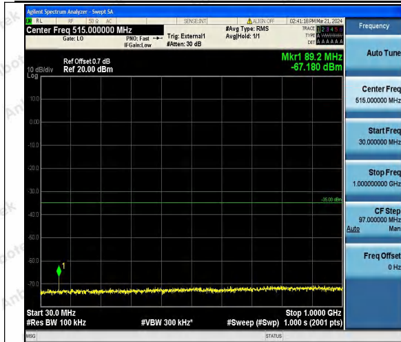
Band41_5MHz_QPSK_41215_1RB#0_30~1000_30~1000
