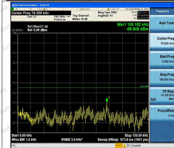
Band41_15MHz_QPSK_40115_1RB#0_0.009~0.15_0 0.009~0.15
