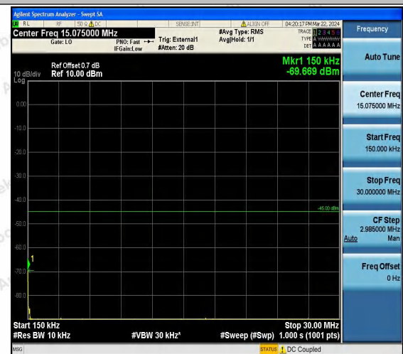
Band41_15MHz_16QAM_40115_1RB#0_0.15~30_0.15~3 0
