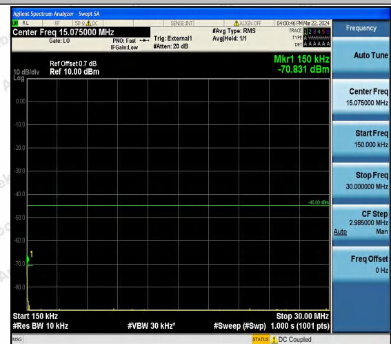
Band41_10MHz_QPSK_41190_1RB#0_0.15~30_0.15~30
