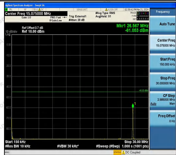
Band41_5MHz_16QAM_40590_1RB#0_0.15~30_0.15~30
