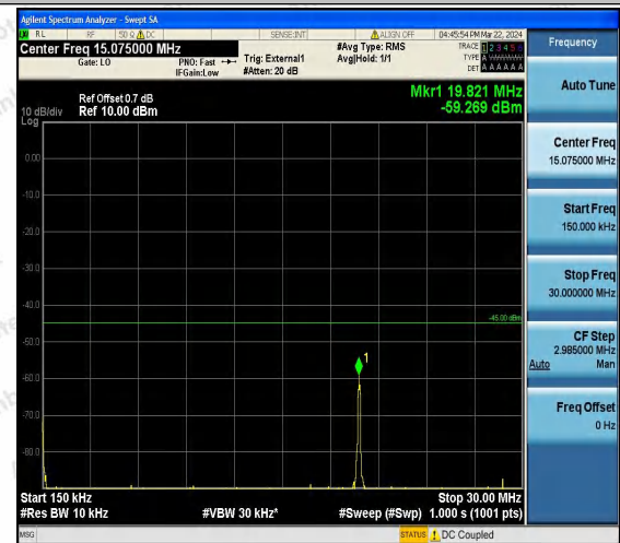
Band41_20MHz_QPSK_40590_1RB#0_0.15~30_0.15~30
