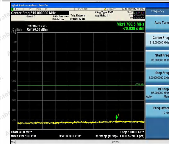
Band41_15MHz_QPSK_40115_1RB#0_30~1000_30~ 1000
