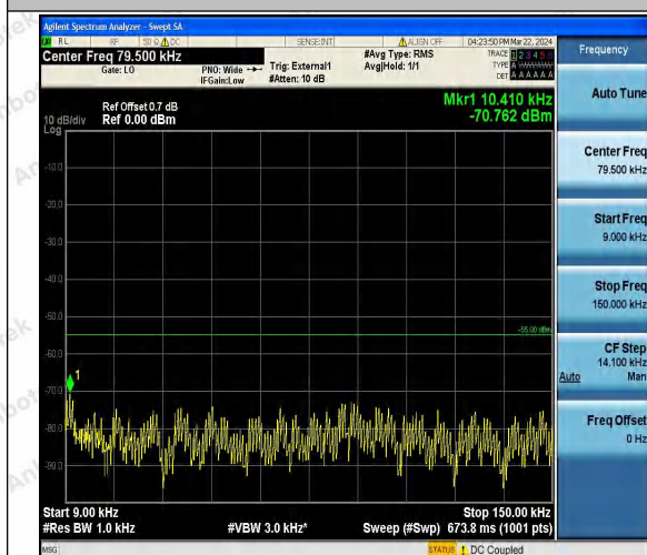
Band41_15MHz_QPSK_41165_1RB#0_0.009~0.15_0 .009~0.15
