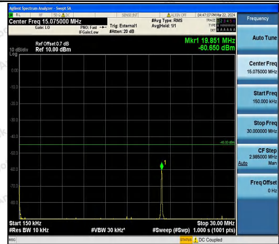
Band41_20MHz_16QAM_40590_1RB#0_0.15~30_0.15~3 0
