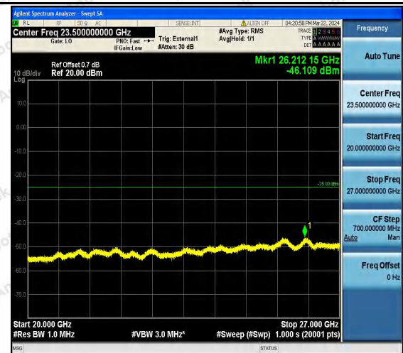
Band41_15MHz_16QAM_40115_1RB#0_20000~27000_2 0000~27000
