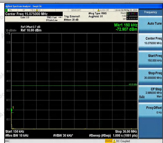
Band41_20MHz_16QAM_40140_1RB#0_0.15~30_0.15~30
