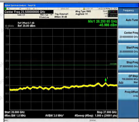
Band41_15MHz_QPSK_40590_1RB#0_20000~27000_20 000~27000
