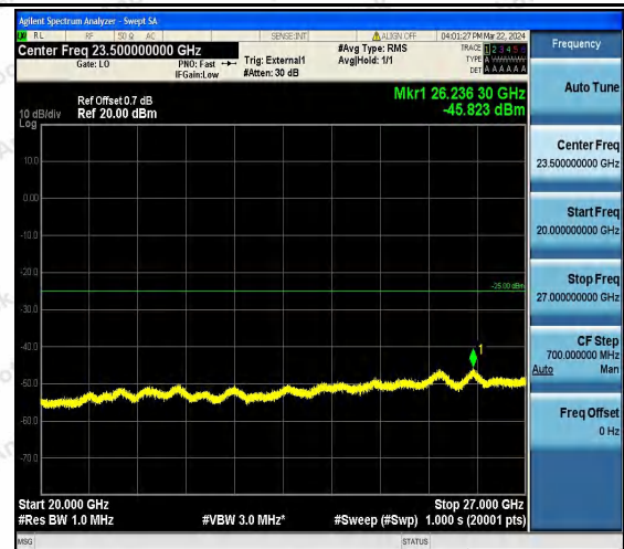
Band41_10MHz_QPSK_41190_1RB#0_20000~27000_20000~27000
