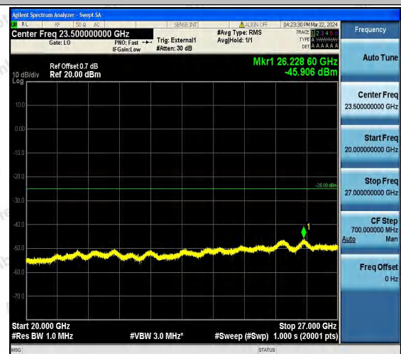
Band41_15MHz_16QAM_40590_1RB#0_20000~27000_2 0000~27000
