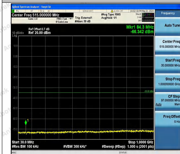
Band41_10MHz_16QAM_41190_1RB#0_30~1000_30~1000
