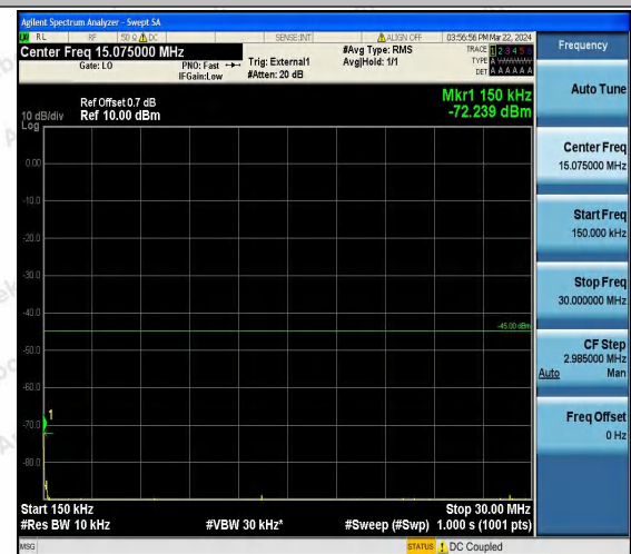
Band41_10MHz_16QAM_40090_1RB#0_0.15~30_0.15~30
