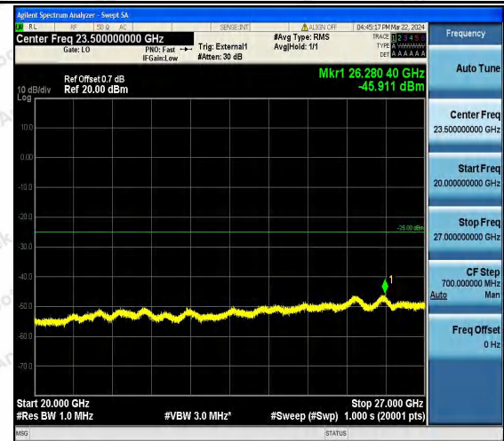
Band41_20MHz_16QAM_40140_1RB#0_20000~27000_2 0000~27000
