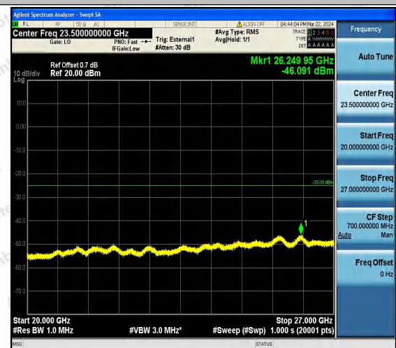
Band41_20MHz_QPSK_40140_1RB#0_20000~27000_20000~27000
