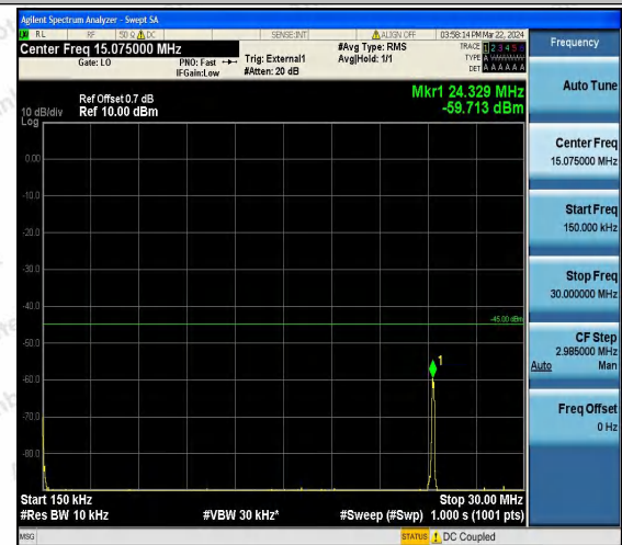
Band41_10MHz_QPSK_40590_1RB#0_0.15~30_0.15~30
