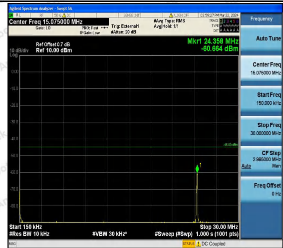
Band41_10MHz_16QAM_40590_1RB#0_0.15~30_0.15~3 0
