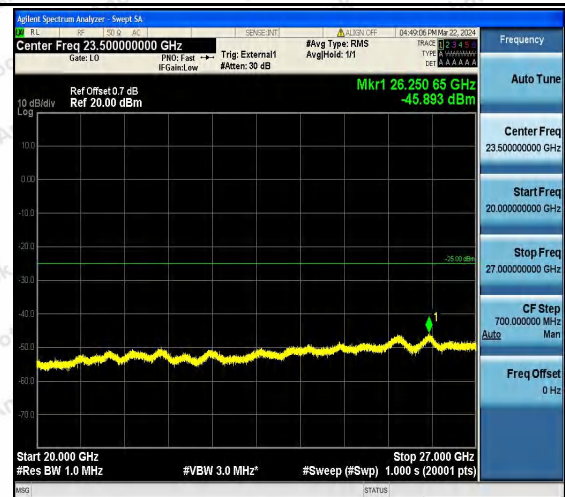
Band41_20MHz_QPSK_41140_1RB#0_20000~27000_20000~27000
