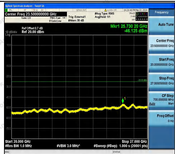
Band41_15MHz_QPSK_41165_1RB#0_20000~27000_20000~27000
