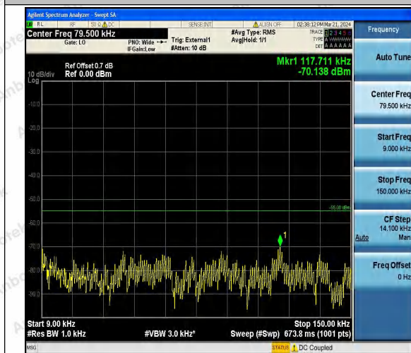
Band41_5MHz_QPSK_40590_1RB#0_0.009~0.15_0 009~0.15
