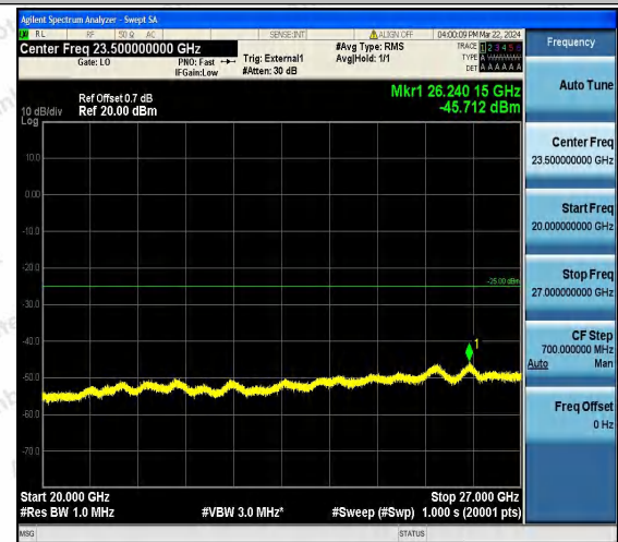
Band41_10MHz_16QAM_40590_1RB#0_20000~27000_2 0000~27000
