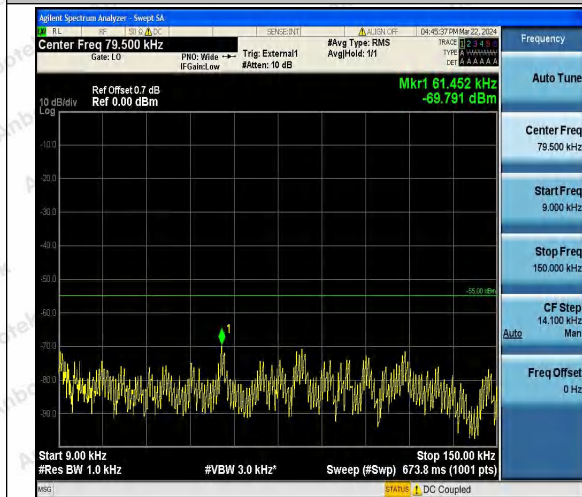
Band41_20MHz_QPSK_40590_1RB#0_0.009~0.15_2 0.009~0.15
