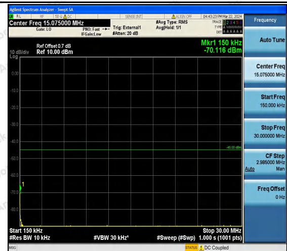
Band41_20MHz_QPSK_40140_1RB#0_0.15~30_0.15~30
