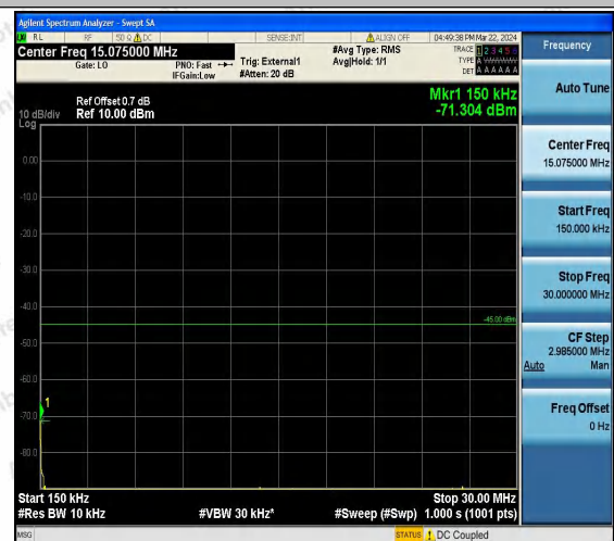
Band41_20MHz_16QAM_41140_1RB#0_0.15~30_0.15~30
