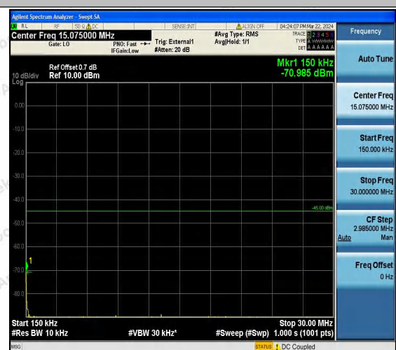
Band41_15MHz_QPSK_41165_1RB#0_0.15~30_0.15~30
