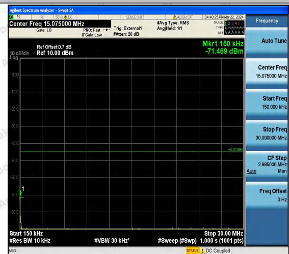
Band41_20MHz_QPSK_41140_1RB#0_0.15~30_0.15~30
