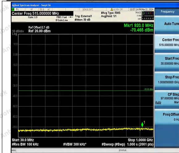
Band41_10MHz_16QAM_40090_1RB#0_30~1000_3 0~1000
