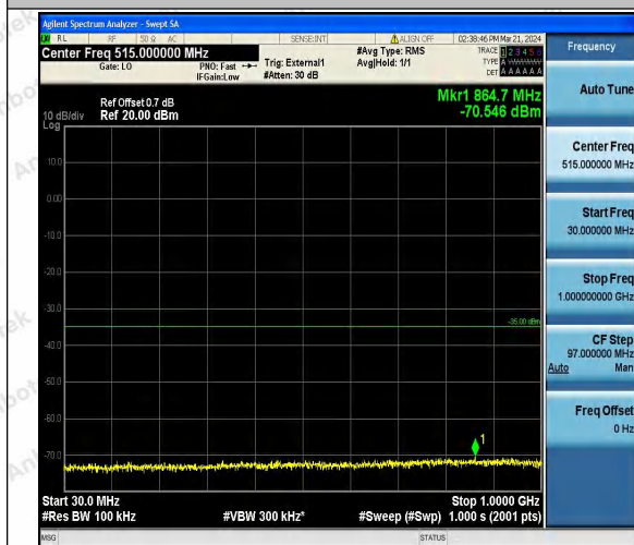
Band41_5MHz_QPSK_40590_1RB#0_30~1000_30~ 1000
