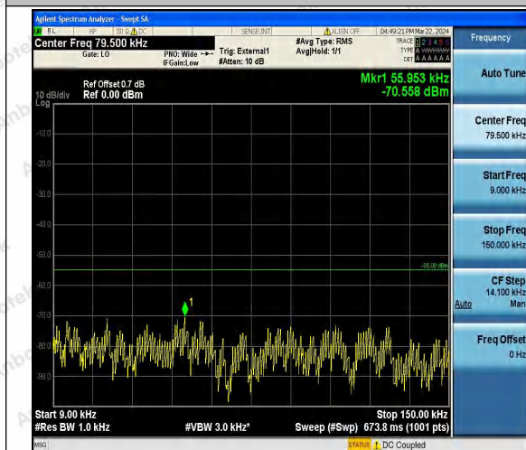
Band41_20MHz_16QAM_41140_1RB#0_0.009~0.15_0.009~0.15
