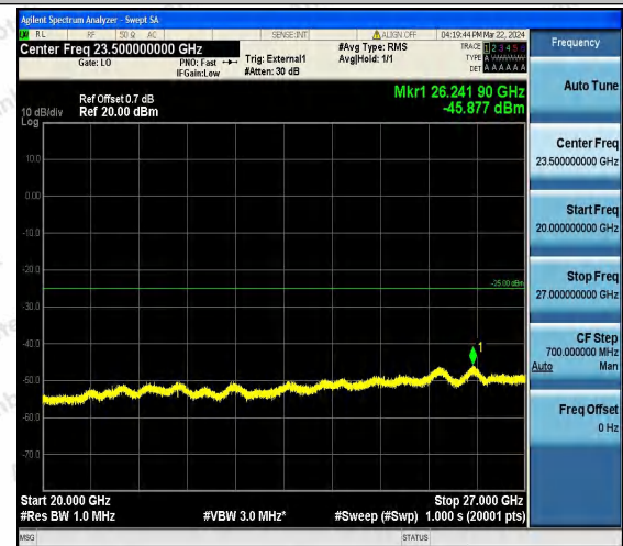
Band41_15MHz_QPSK_40115_1RB#0_20000~27000_20 000~27000
