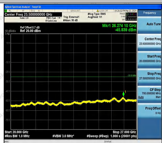
Band41_15MHz_16QAM_41165_1RB#0_20000~27000_20000~27000
