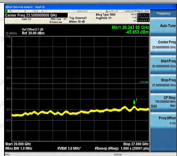
Band41_10MHz_16QAM_41190_1RB#0_20000~27000_20000~27000
