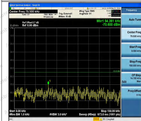
Band41_15MHz_QPSK_40590_1RB#0_0.009~0.15_0.009~0.15
