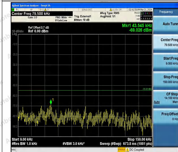
Band41_5MHz_16QAM_41215_1RB#0_0.009~0.15_0.009~0.15
