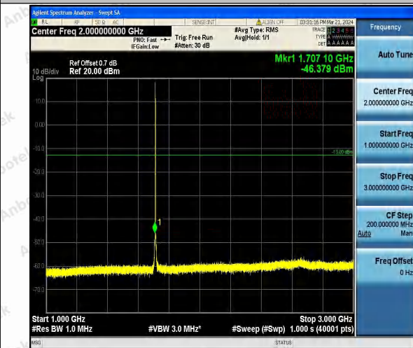
Band66_1.4MHz_QPSK_131979_1RB#0_1000~3000_1000~3000
