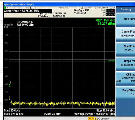
Band66_1.4MHz_QPSK_132665_1RB#0_0.15~30.0.15~30
