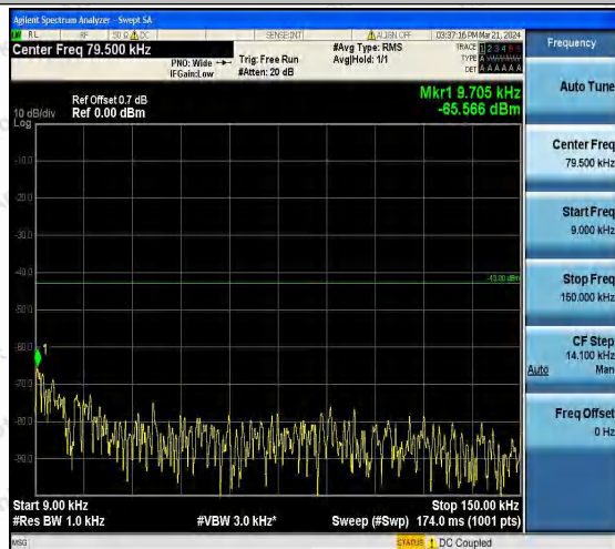
Band66_1.4MHz_QPSK_132665_1RB#0_0.009~0.15_0.009~0.15
