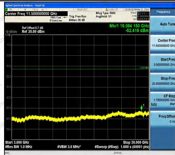
Band66_1.4MHz_16QAM_132322_1RB#0_3000~20000_3000~20000
