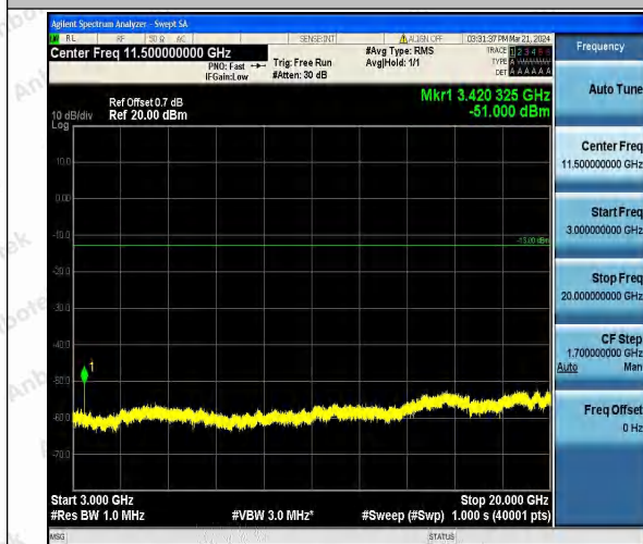
Band66_1.4MHz_QPSK_131979_1RB#0_3000~20000_3000~20000
