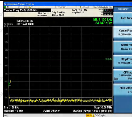
Band66_5MHz_QPSK_131997_1RB#0_0.15~30_0.15~30 0
