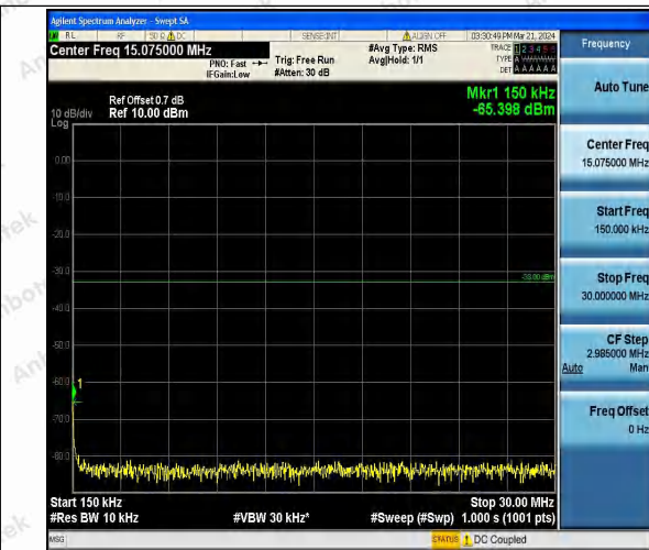
Band66_1.4MHz_QPSK_131979_1RB#0_0.15~30_0.15~30
