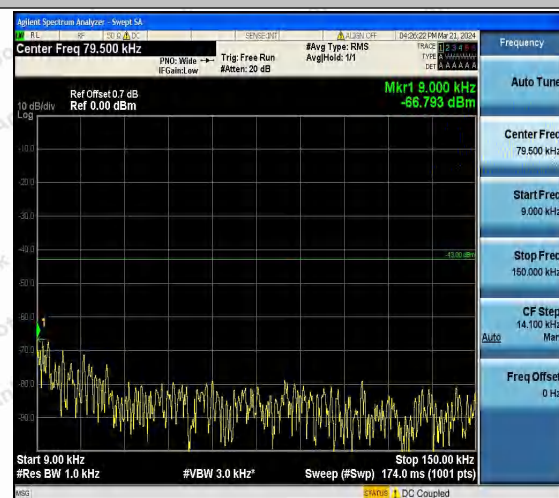
Band66_5MHz_16QAM_131997_1RB#0_0.009~0.15_0. 009~0.15
