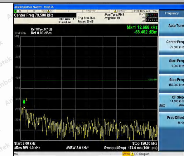
Band66_1.4MHz_16QAM_131979_1RB#0_0.009~0.15_0.009~0.15
