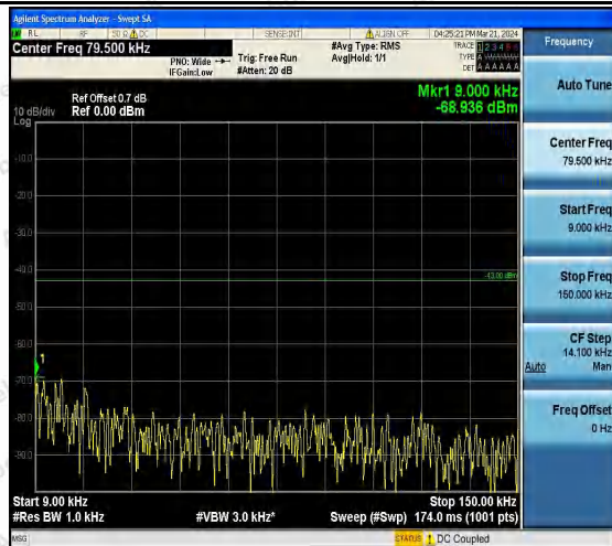
Band66_5MHz_QPSK_131997_1RB#0_0.009~0.15_0. 009~0.15
