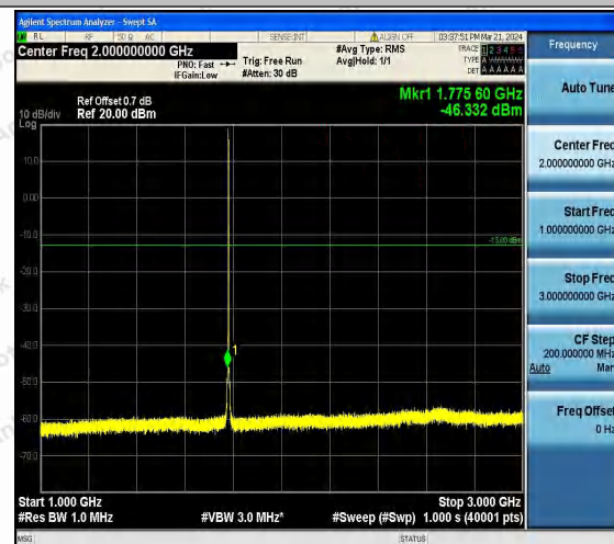
Band66_1.4MHz_QPSK_132665_1RB#0_1000~3000.1000~3000
