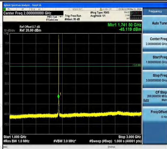
Band66_1.4MHz_16QAM_132322_1RB#0_1000~3000_1000~3000
