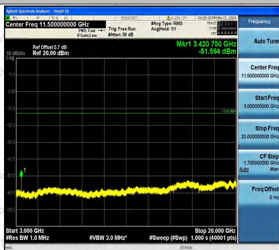
Band66_5MHz_QPSK_131997_1RB#0_3000~20000_3 000~20000
