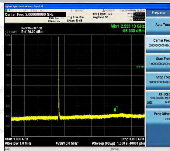
Band66_5MHz_QPSK_131997_1RB#0_1000~3000_100 0~3000
