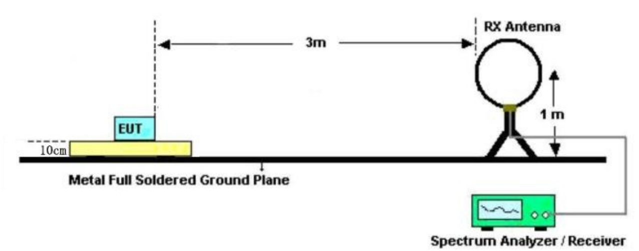
Figure 1. Below 30MHz
