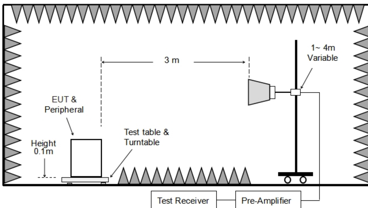
Figure 3. Above 1 GHz
