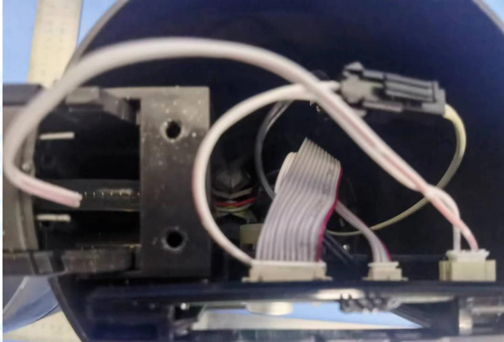
Photo 10 Internal of EUT
