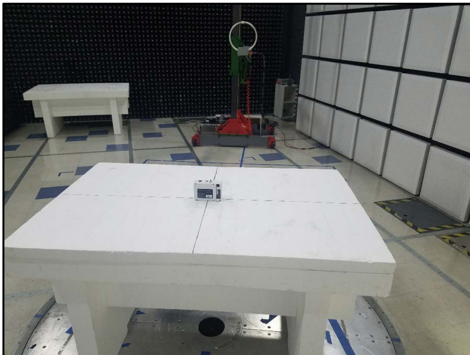
Radiated Emissions-6
