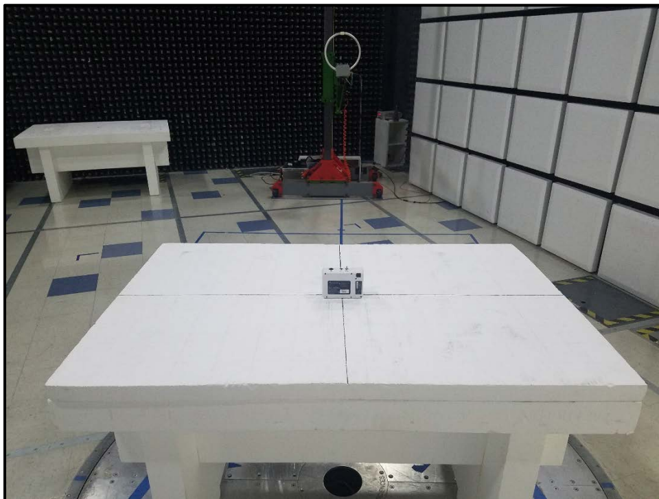
Radiated Emissions-4
