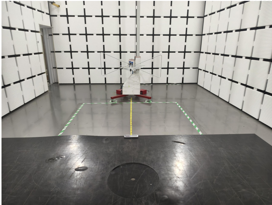
Radiated Emission Test (In Semi Anechoic Chamber)
