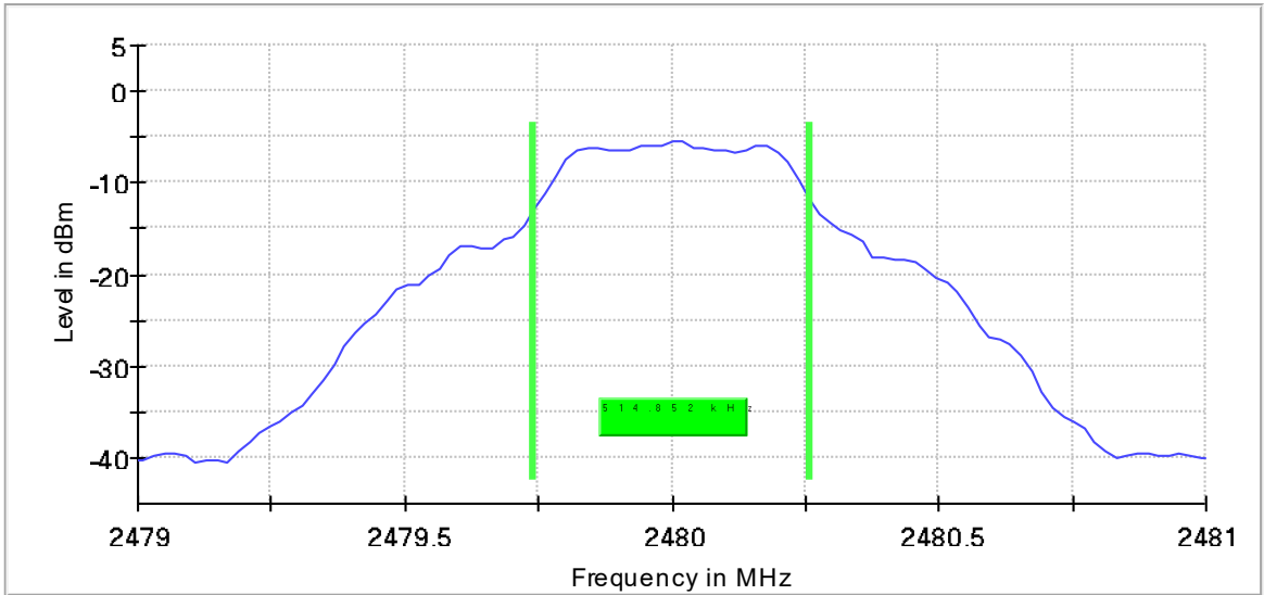
6 dB Bandwidth
