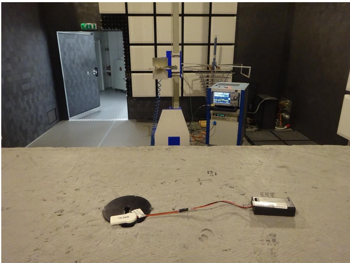
Figure 4: Spurious emission 1 GHz - 18 GHz
