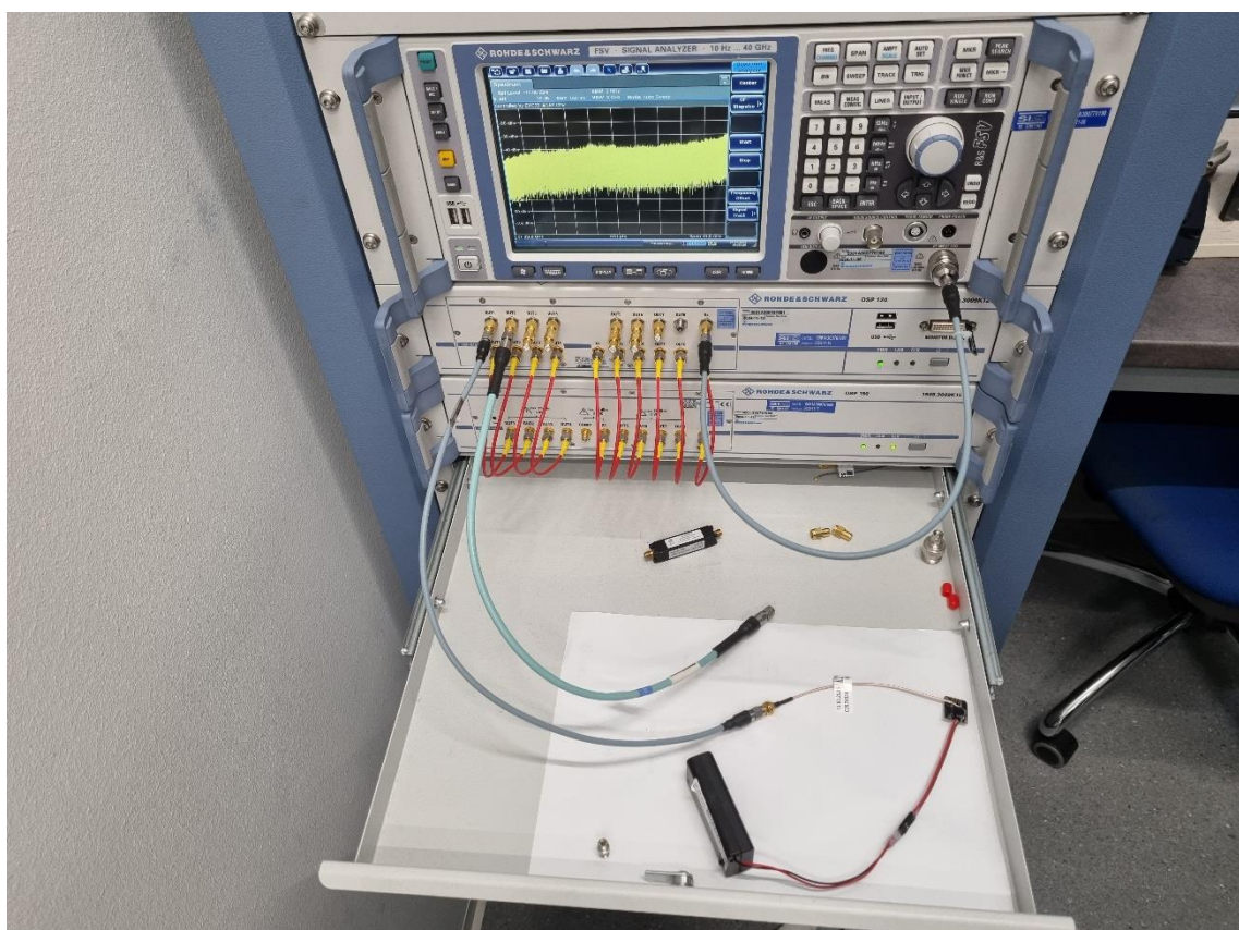
Figure 6: Conducted measurements test setup
