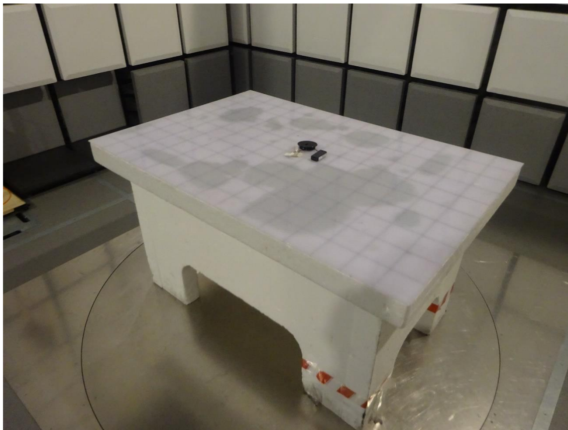
Figure 1: Radiated emission
