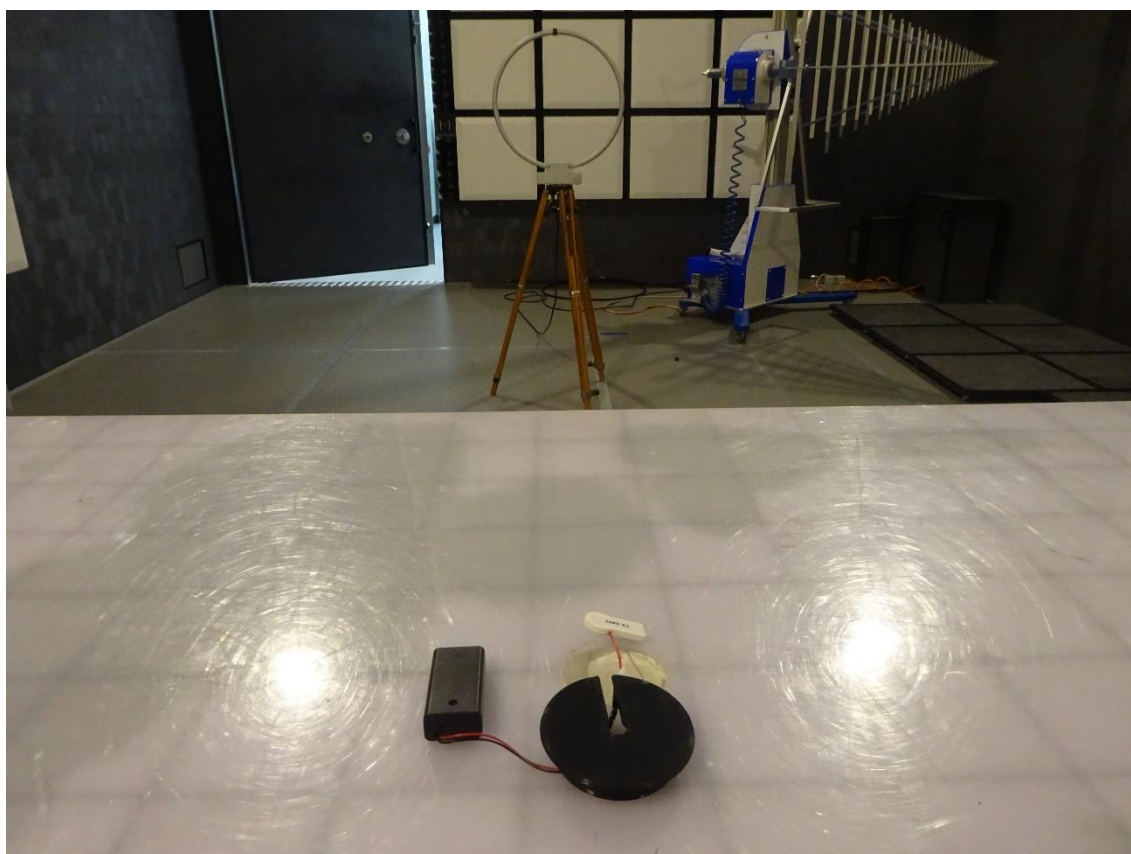
Figure 2: Radiated Spurious emission 90 kHz - 30 MHz
