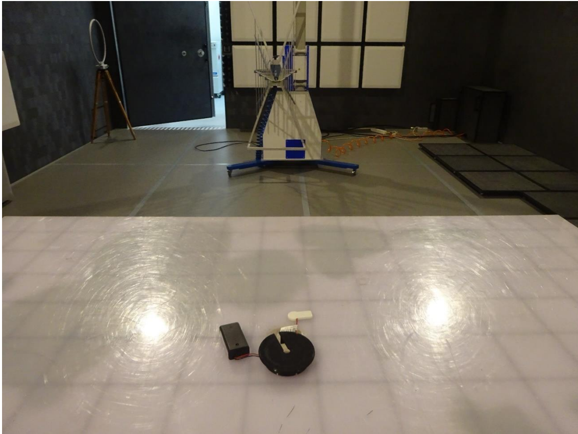
Figure 3: Spurious emission 30 MHz - 1000 MHz
