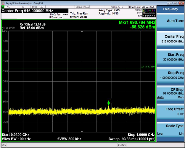
11AX40SISO-Ant1-2452-30~1000-PASS
