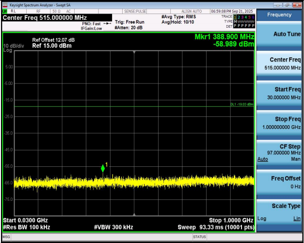
11AX20SISO-Ant1-2462-30~1000-PASS
