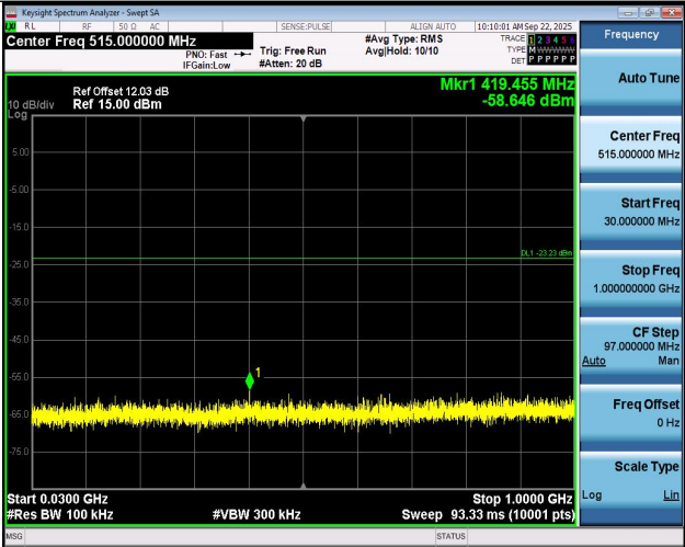
11AX40SISO-Ant1-2437-30~1000-PASS
