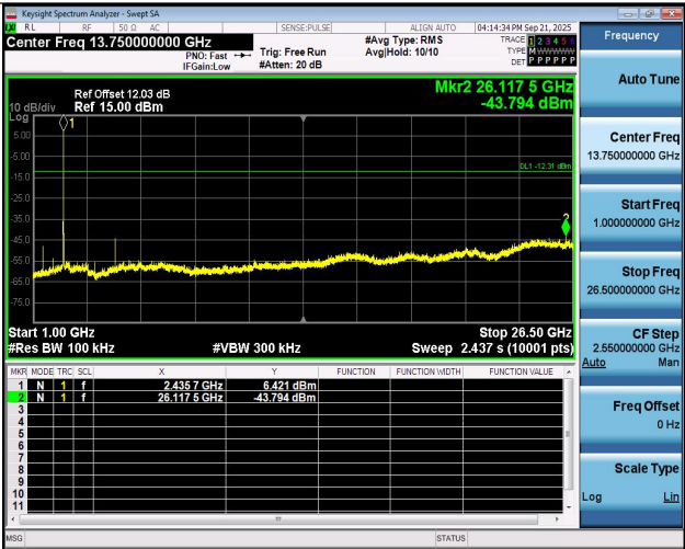
11B-Ant1-2437-1000~26500-PASS
