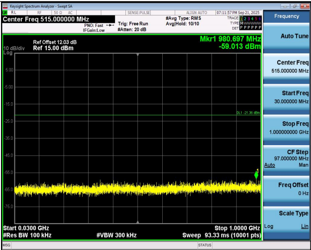
11AX40SISO-Ant1-2422-30~1000-PASS
