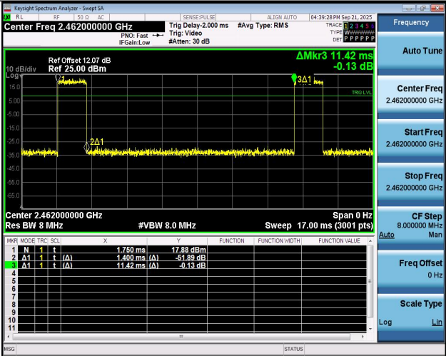
NTNV-11G-Ant1-2462
