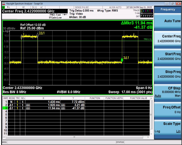
NTNV-11AX40SISO-Ant1-2422
