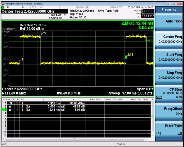
NTNV-11N40SISO-Ant1-2422
