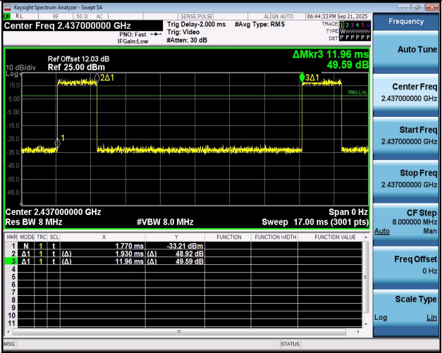
NTNV-11AX20SISO-Ant1-2437
