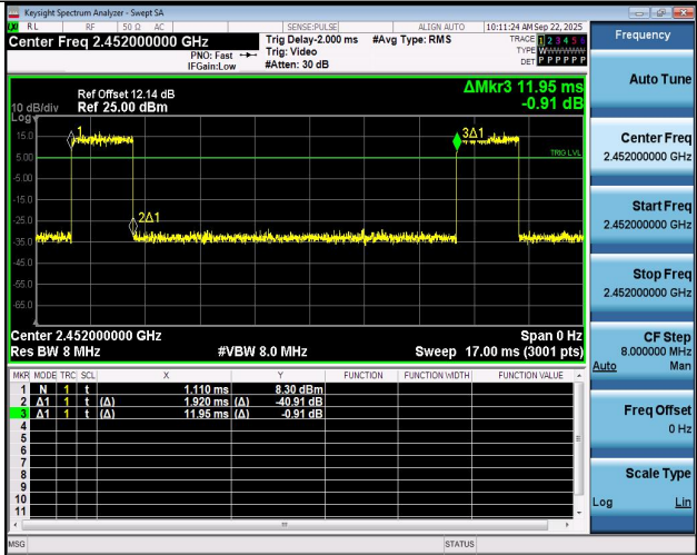
NTNV-11AX40SISO-Ant1-2452
