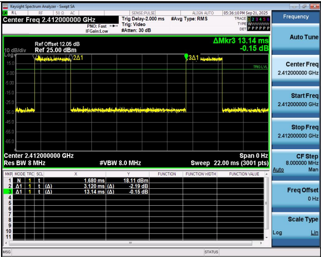
NTNV-11N20SISO-Ant1-2412
