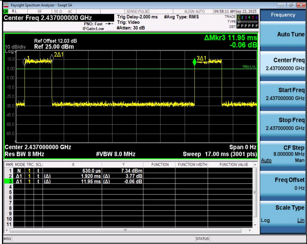
NTNV-11AX40SISO-Ant1-2437
