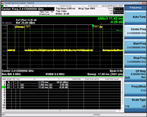
NTNV-11G-Ant1-2412
