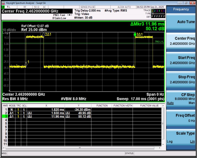
NTNV-11AX20SISO-Ant1-2462
