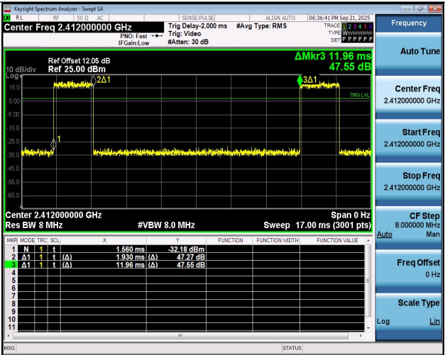
NTNV-11AX20SISO-Ant1-2412
