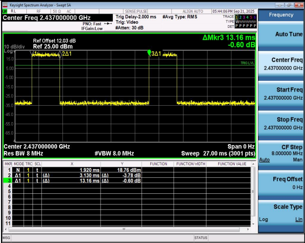
NTNV-11N20SISO-Ant1-2437
