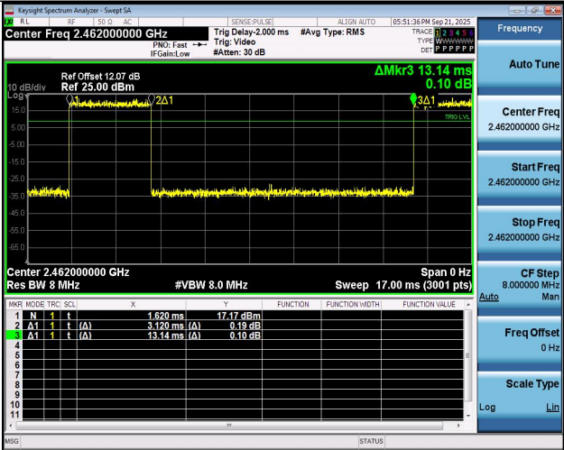
NTNV-11N20SISO-Ant1-2462
