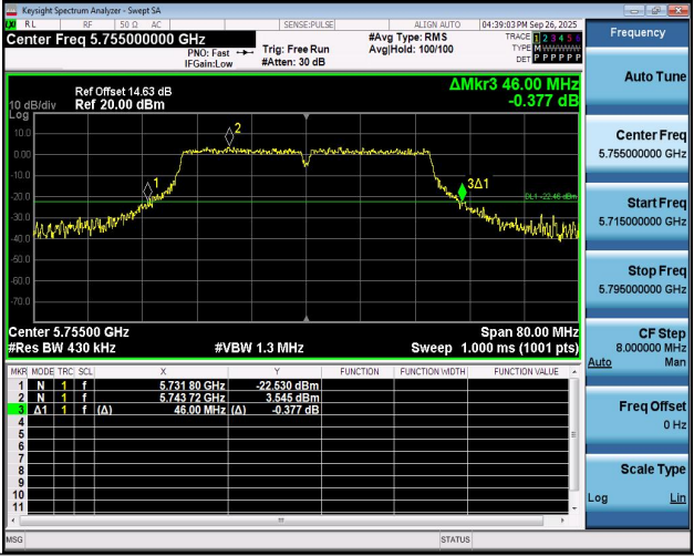
11N40SISO-Ant1-5755
