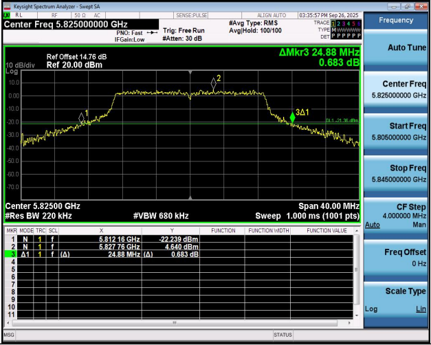
11N20SISO-Ant1-5825
