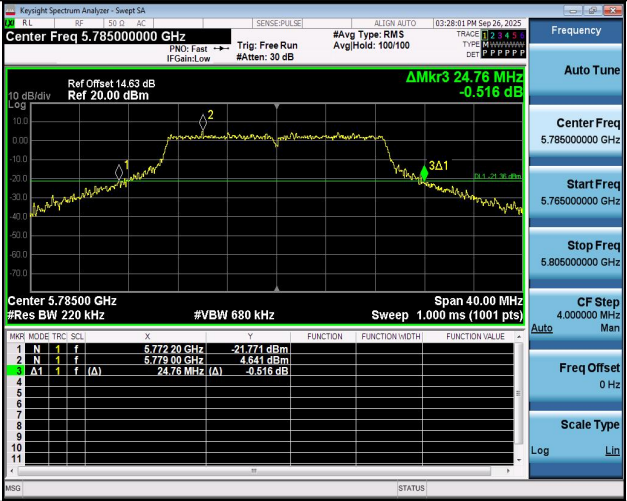
11N20SISO-Ant1-5785
