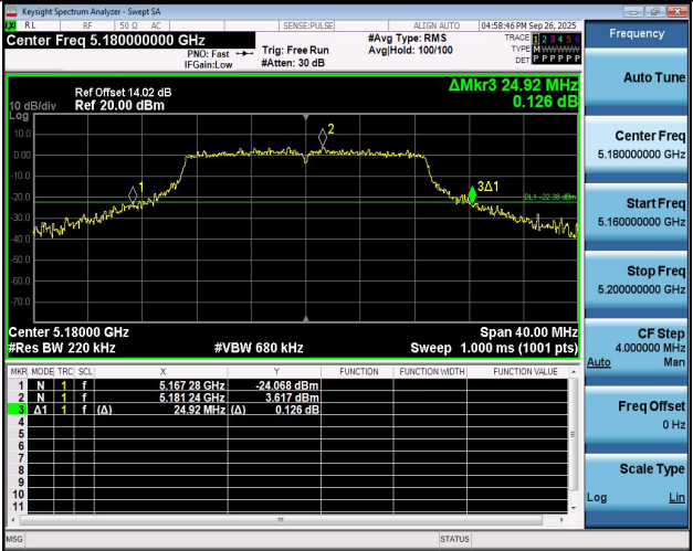
11AC20SISO-Ant1-5180
