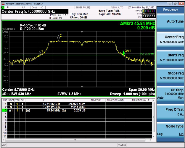
11AC40SISO-Ant1-5755
