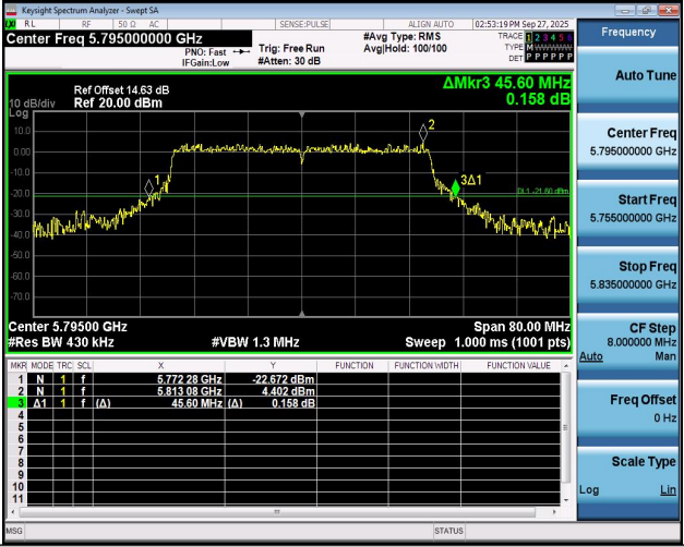
11AX40SISO-Ant1-5795
