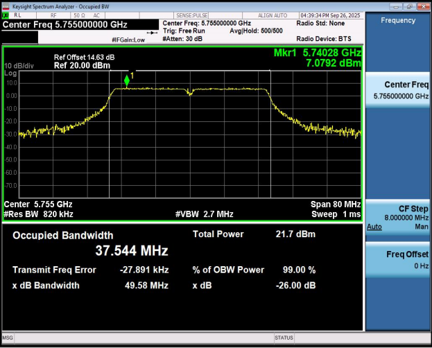
11N40SISO-Ant1-5755
