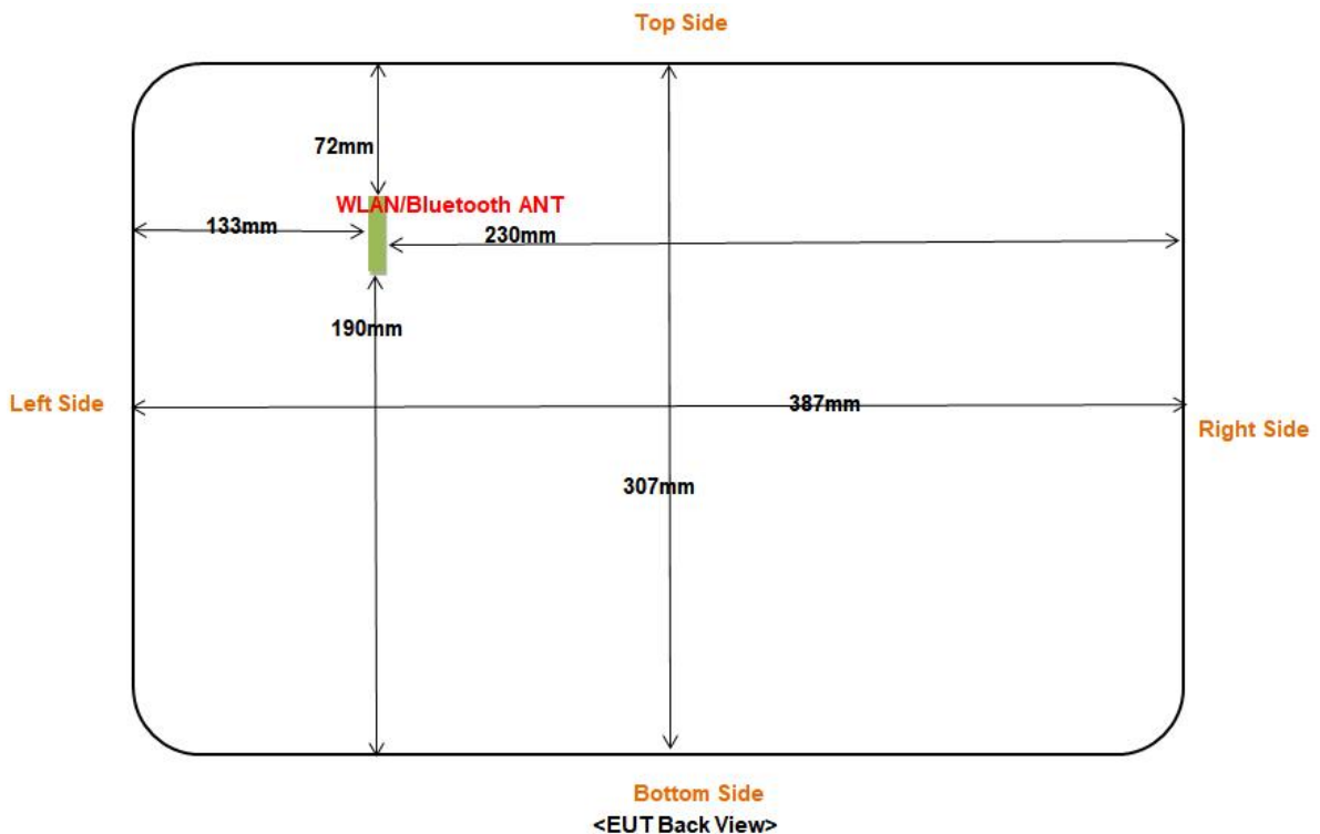
Fig 7.2 Block Diagram for EUT Antenna Position
