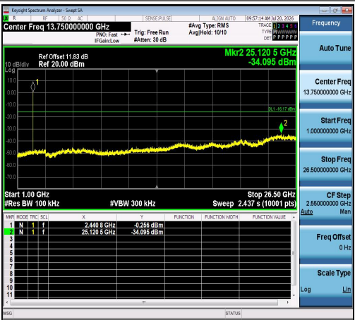
LE_2M-Ant1-2440-1000~26500-PASS
