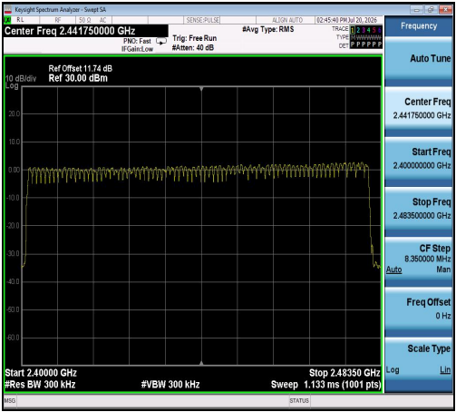
3DH5-Ant1-Hop-PASS
