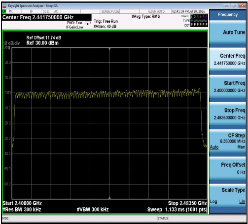
2DH5-Ant1-Hop-PASS
