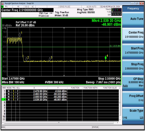
3DH5-Ant1-Hop_2480-PASS
