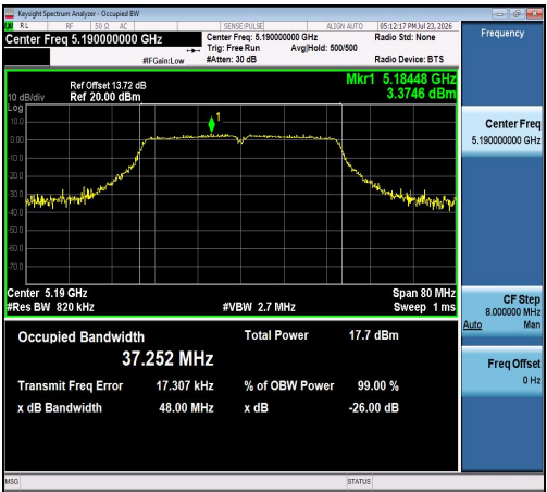
11N40SISO-Ant1-5190
