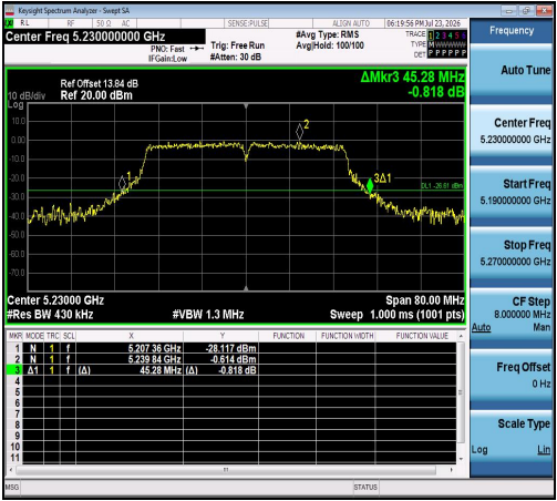
11AC40SISO-Ant1-5230
