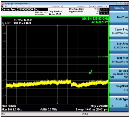
11AX40SISO-Ant1-5795-30~5650-PASS
