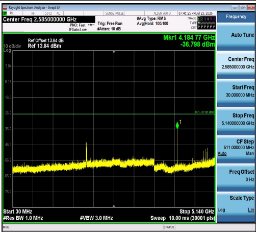
11AX40SISO-Ant1-5230-30~5140-PASS
