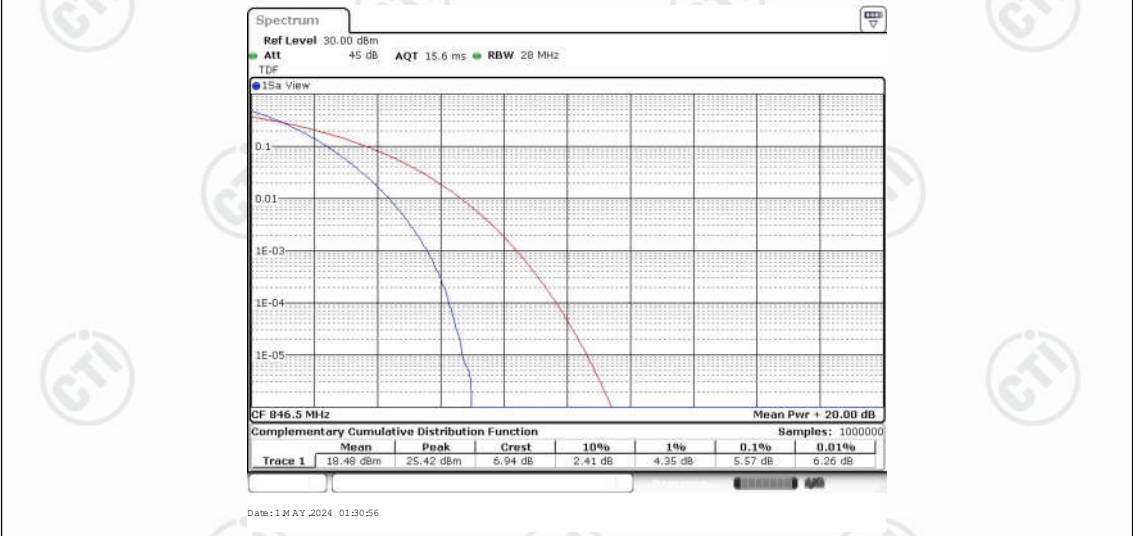
Band26-5MHz-QPSK-27015-25RB#0
