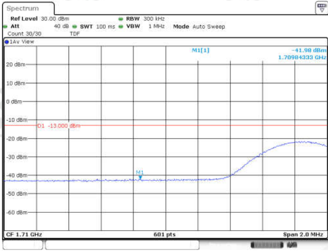
Band4-15MHz-16QAM-20025-1RB#74
