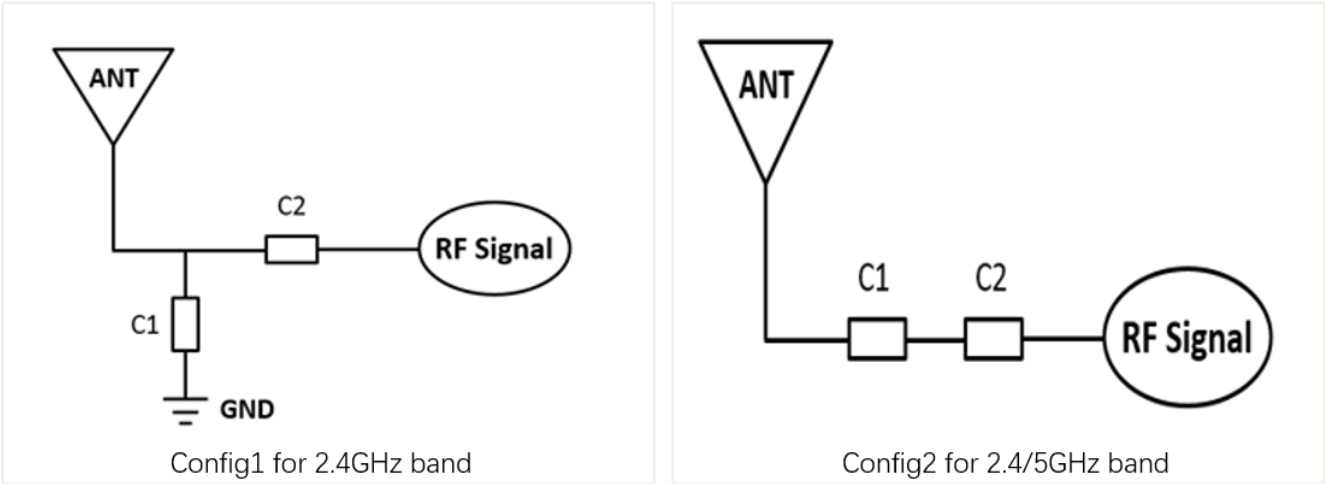
FIGURE 5.1 RECOMMENDED MATCHING CIRCUIT SCHEMATIC FOR CONFIGURE 1 AND CONFIGURE 2
