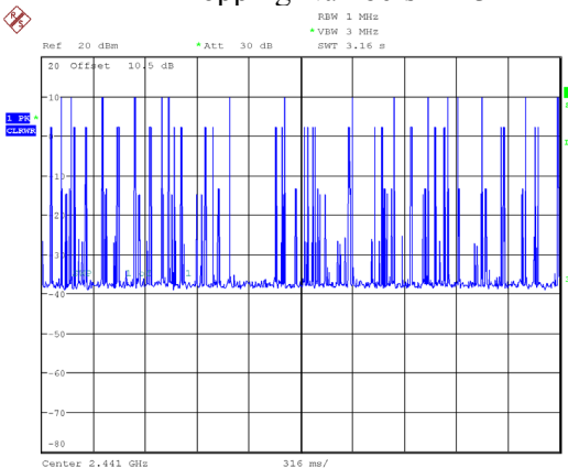
Hopping Numbers-DH3
