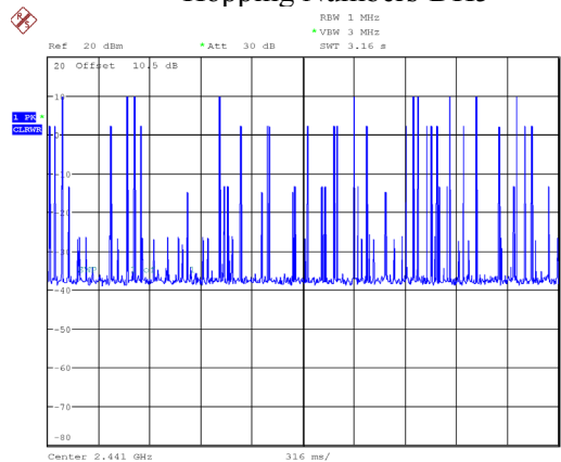
Hopping Numbers-DH5
