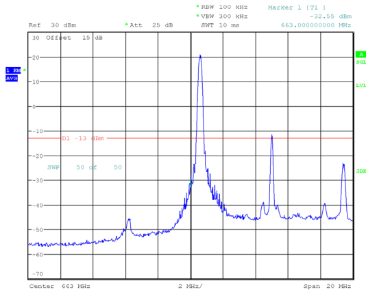
10 MHz_Low_QPSK_RB1#0
