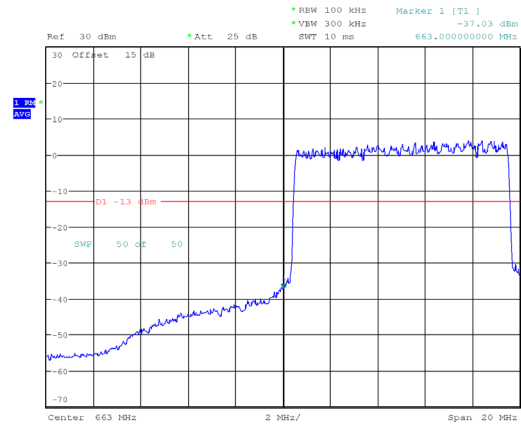
10 MHz_Low_QPSK_RB50#0
