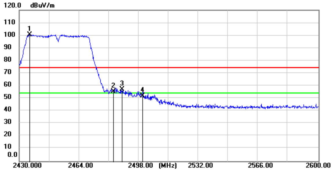
11n(HT40)_TX_CH_09_Vertical_Peak
