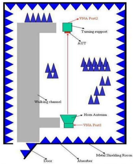
The Environment of Antenna Radiation Pattern
