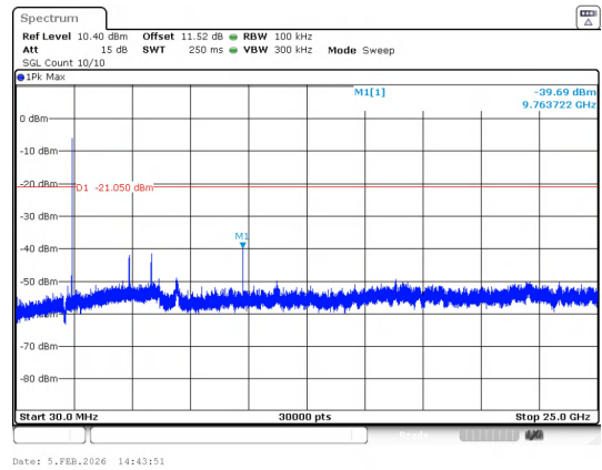
30.0 MHz - 25000.0 MHz π/4DQPSK_2-DH5_Channel 39
