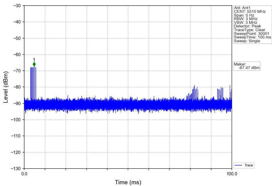
Signal Calibration_802.11n(HT40)_2C_5510MHz_RadarType6_Trial0
