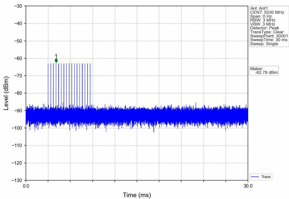
Signal Calibration_802.11ac(VHT80)_2C_5530MHz_RadarType3_Trial0
