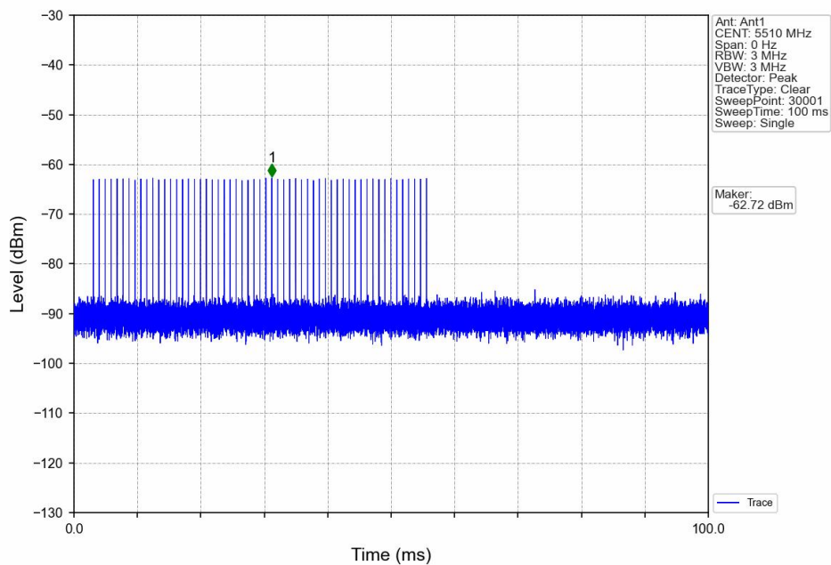
Signal Calibration_802.11n(HT40)_2C_5510MHz_RadarType2_Trial0
