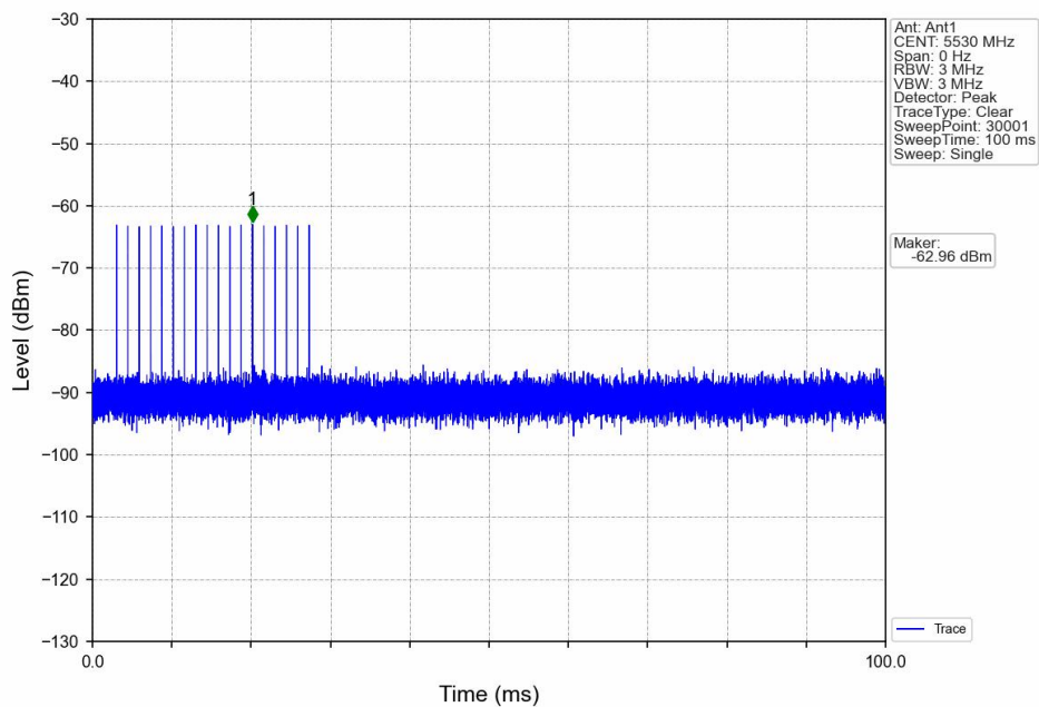
Signal Calibration_802.11ac(VHT80)_2C_5530MHz_RadarType1_Trial0
