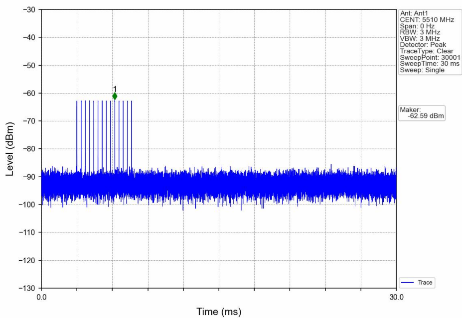
Signal Calibration_802.11n(HT40)_2C_5510MHz_RadarType4_Trial0
