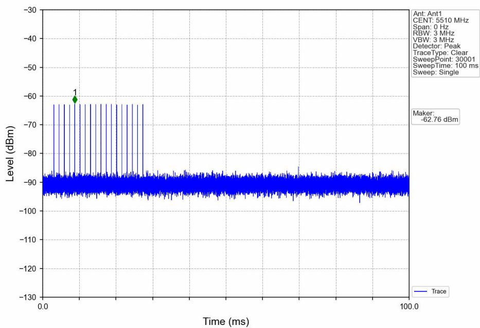
Signal Calibration_802.11n(HT40)_2C_5510MHz_RadarType0_Trial0
