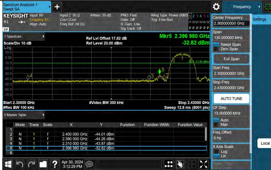
11B-Ant2-2412-PASS
