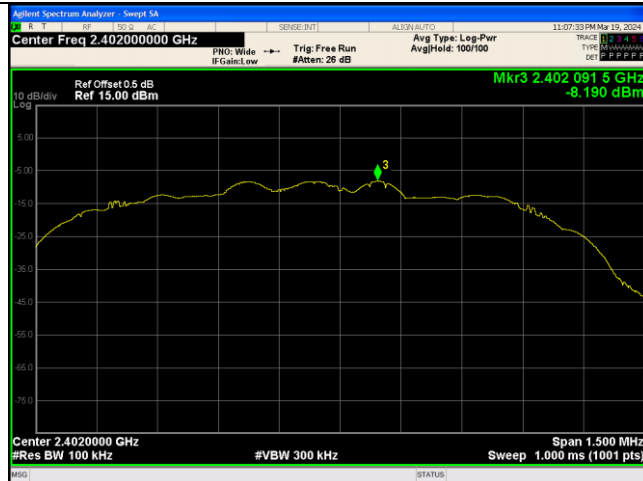
In-Band Reference Level 8DPSK 3-DH5 Channel 0
