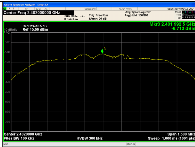
In-Band Reference Level \pi/4 DQPSK 2-DH5 Channel 0
