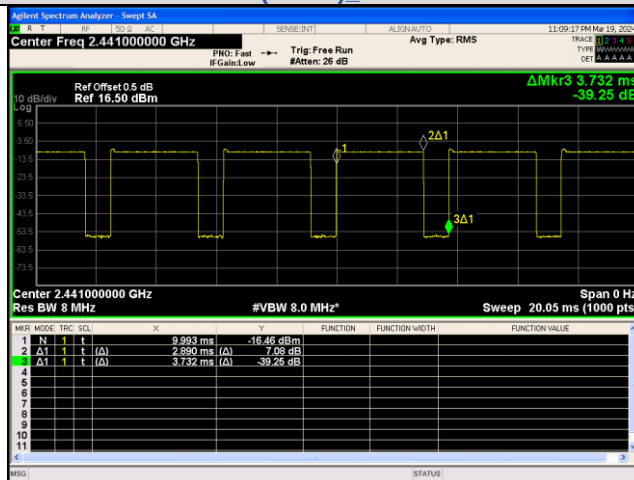
8DPSK(3-DH5) Channel 39
