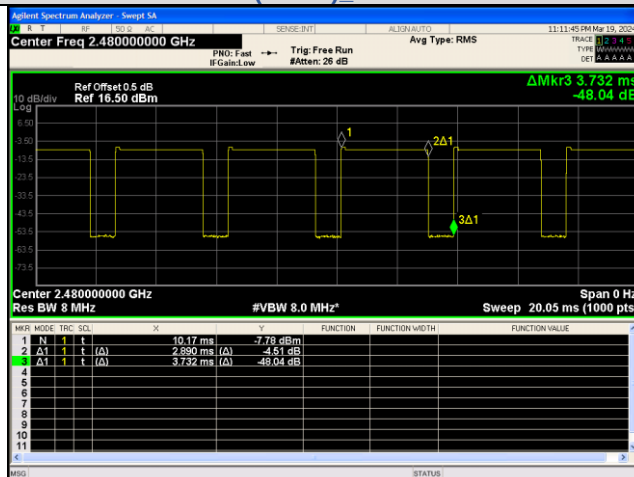
8DPSK(3-DH5) Channel 78
