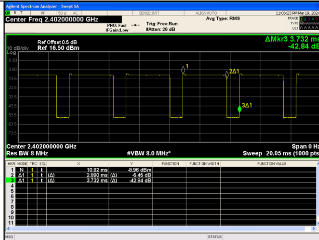
8DPSK(3-DH5) Channel 0
