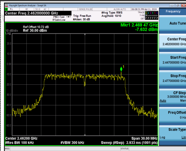
Reference CH11
